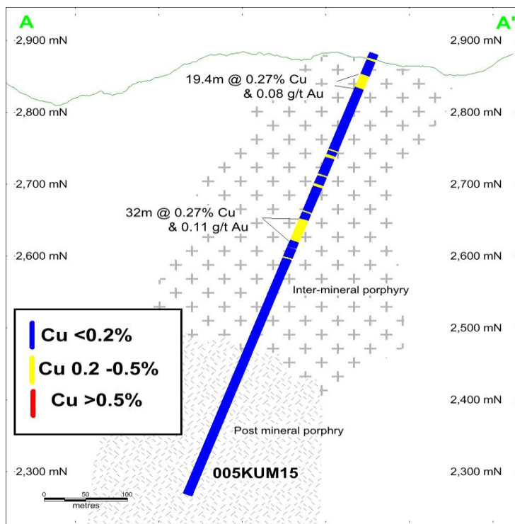
Section view of Kum Kom drilling
