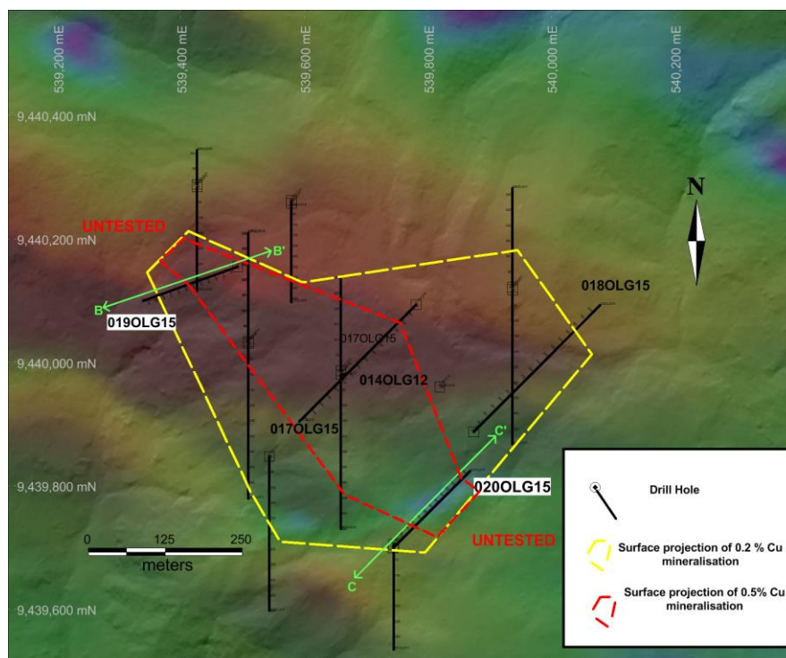
Plan view of Olgal drill holes
