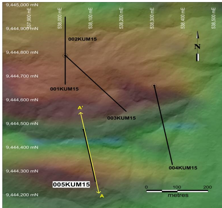
Plan view of Kum Kom drilling
