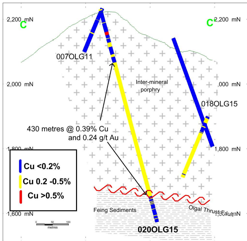
Section view of Olgal drill holes 18 and 20
