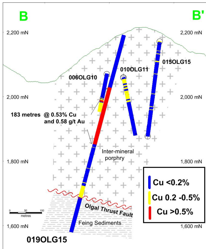
Section view of Olgal hole 19
