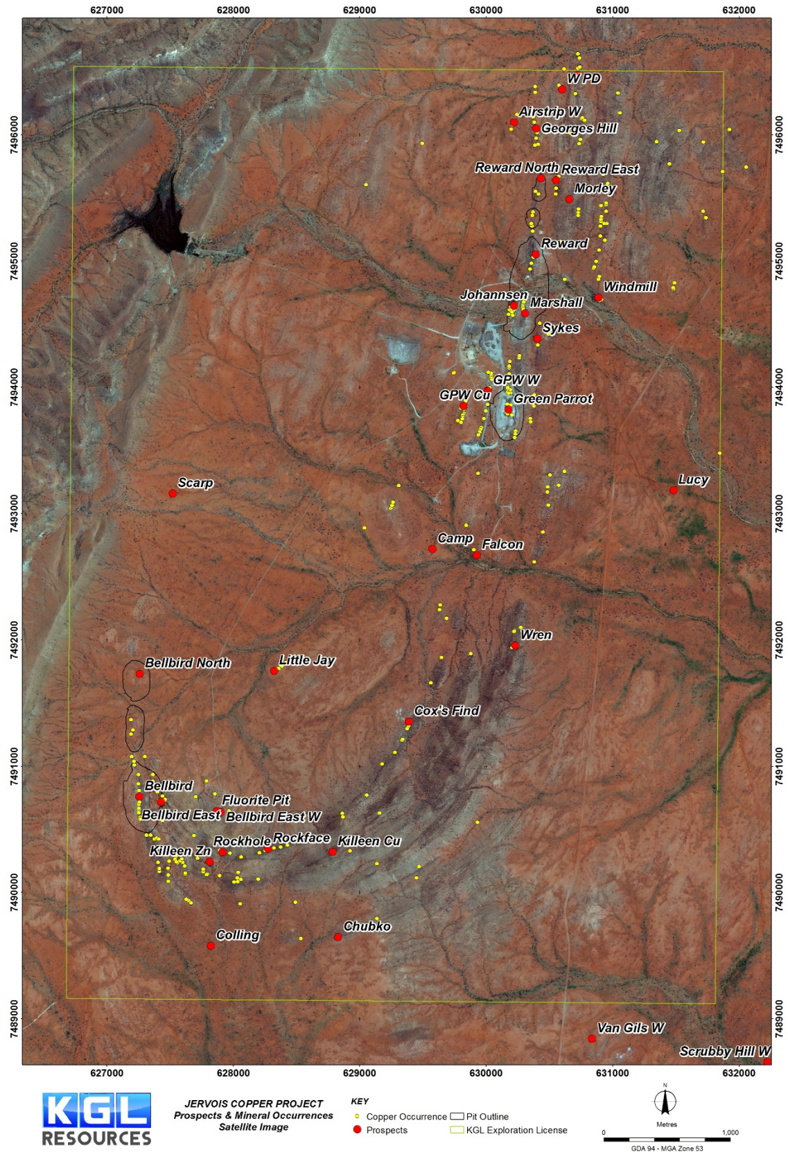
FIGURE 4 JERVOIS PROJECT PROSPECT LOCATION
