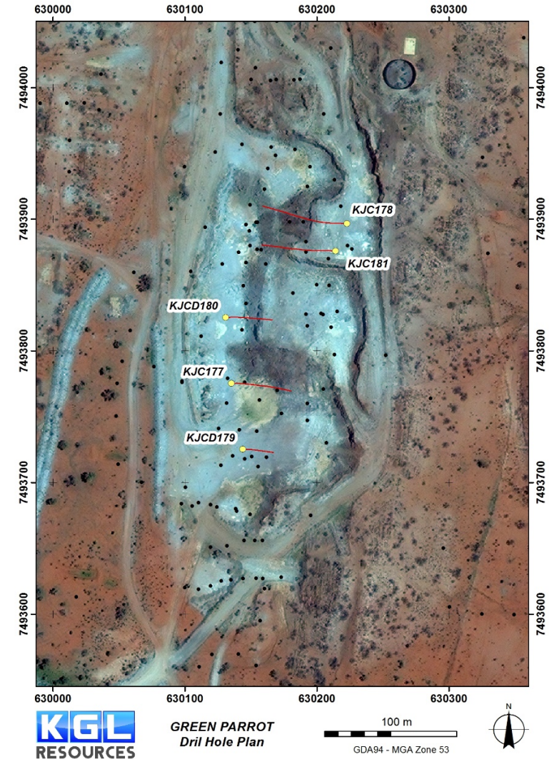
FIGURE 3 PLAN OF DIAMOND AND RC DRILLING
