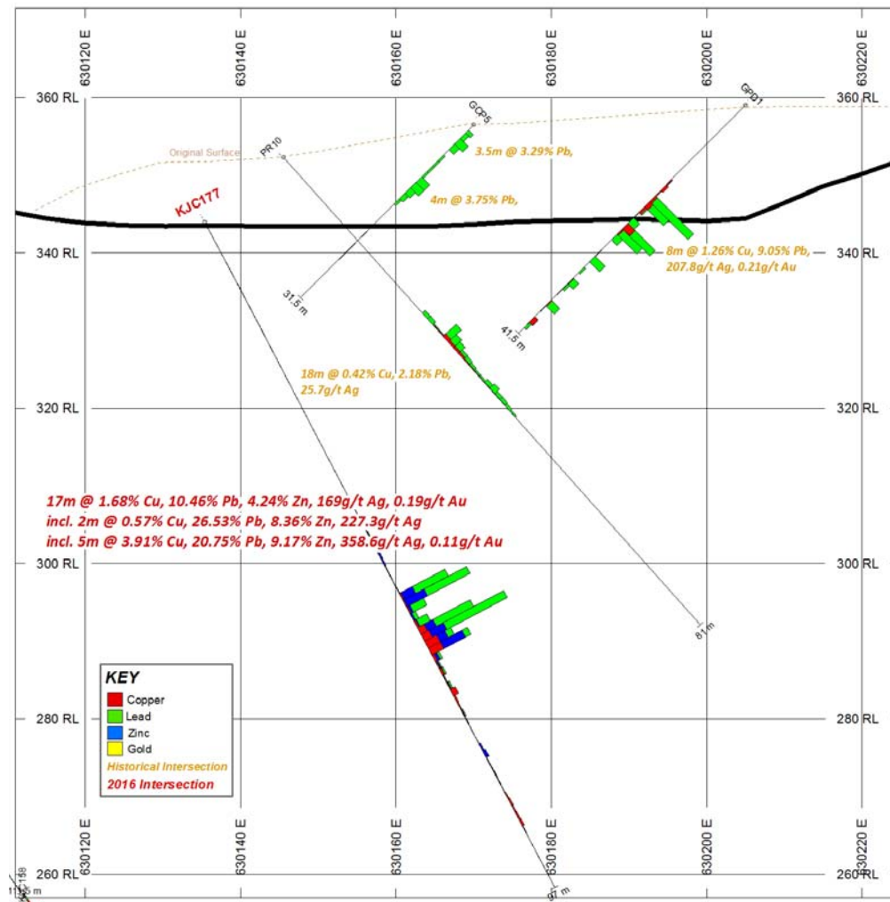
FIGURE 2 GREEN PARROT PROSPECT CROSS SECTION 7493770N (12M WINDOW)
