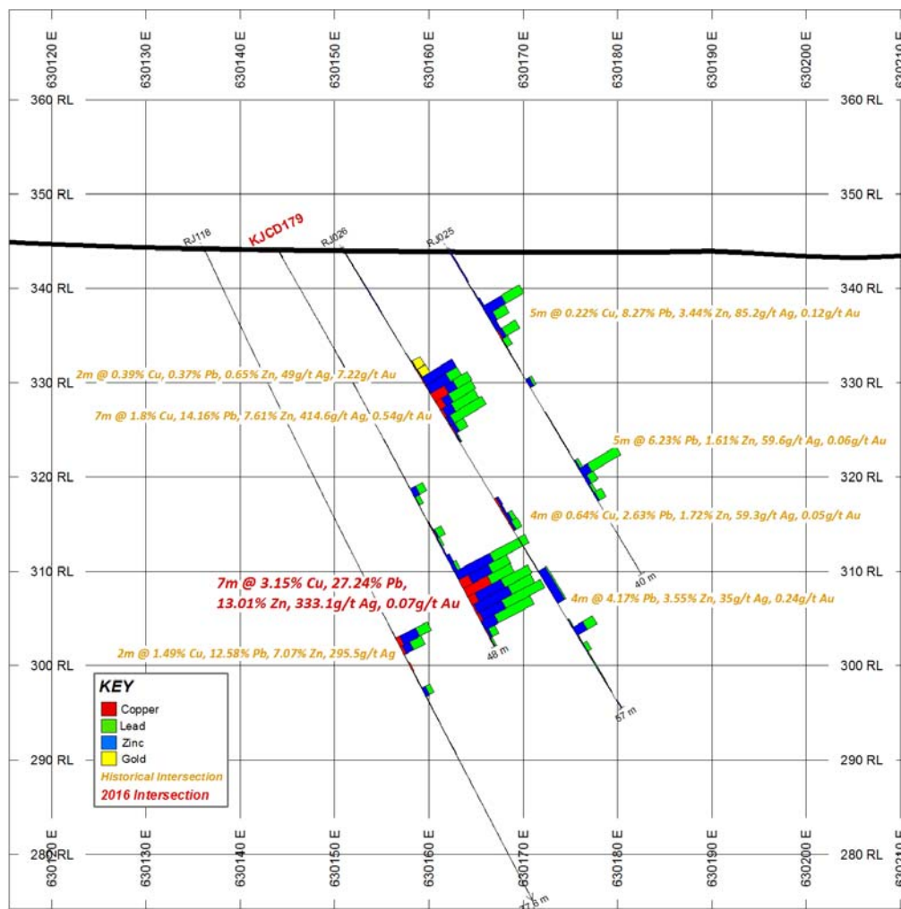
FIGURE 1 GREEN PARROT PROSPECT CROSS SECTION 7493720N (12M WINDOW)
