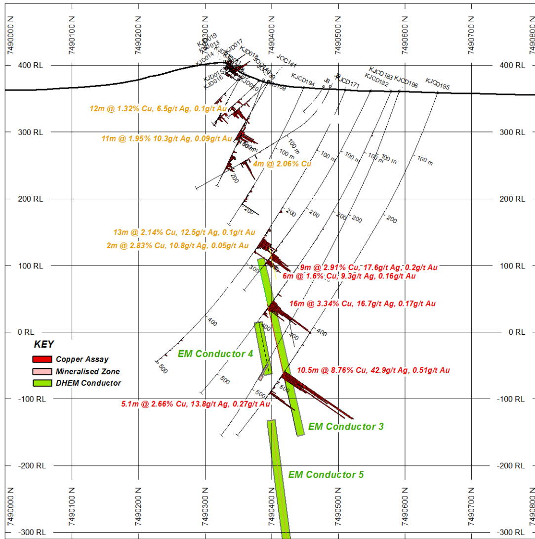
Figure 3 Cross section 628 300E (200m section window)
