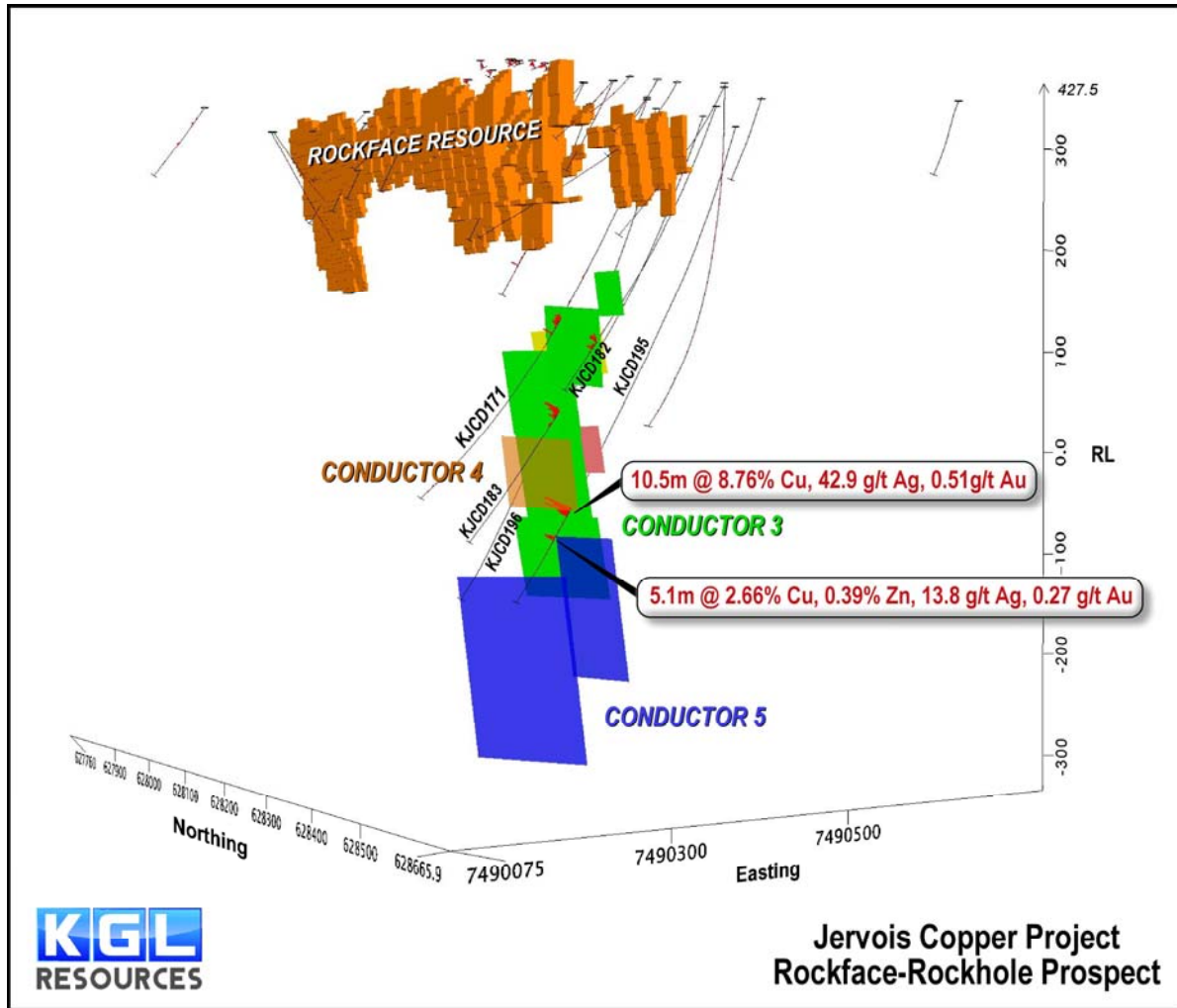
Figure 1 Rockface Prospect DHEM conductive plates
