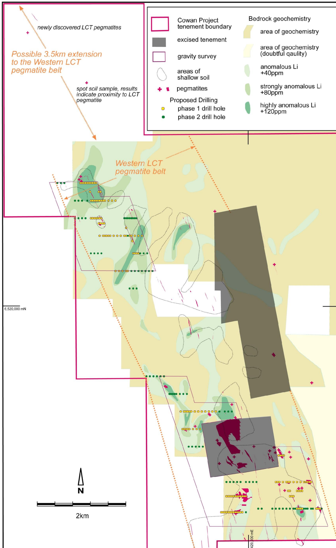
Figure 3 | Enlargement, proposed drill locations
