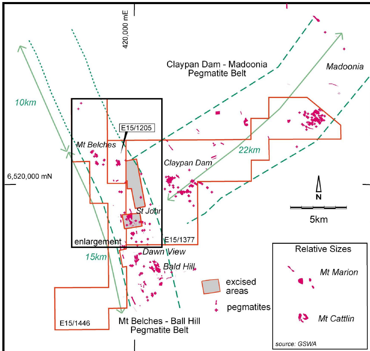
Figure 2 | Known pegmatite belts within Cowan Project area
