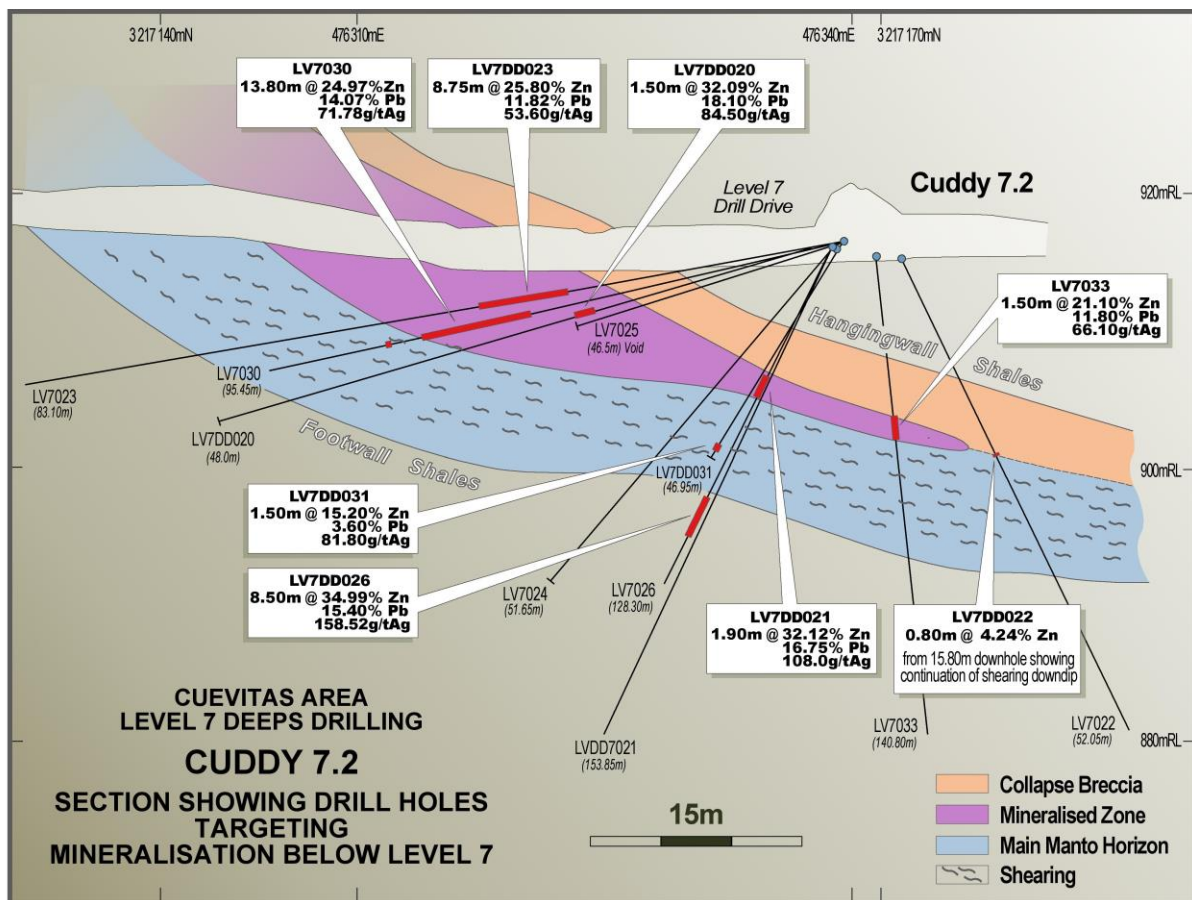
Figure 2. Drilling completed from Cuddy 7.2 with drilling results to date. Several holes are out of plane of the section and may be as much as 70m off section (refer to Figure 1)
