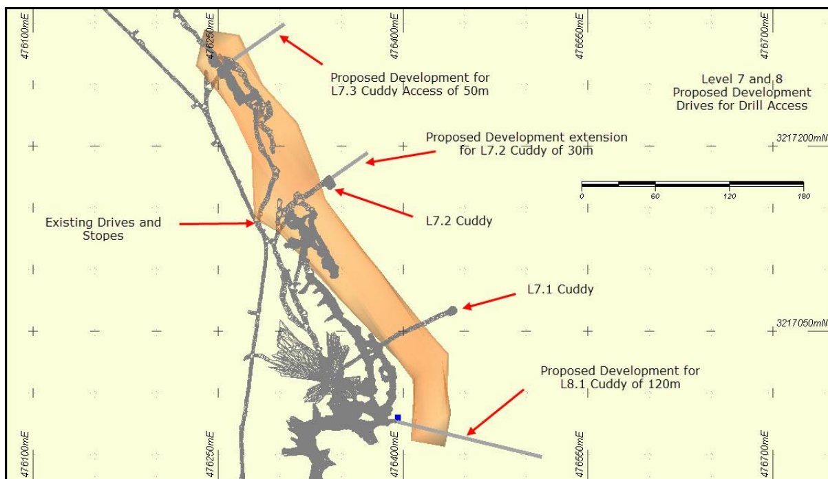
Figure 3. Proposed development locations from Level 7 opening up the down dip and northern and southern extensions of the mineralisation.
