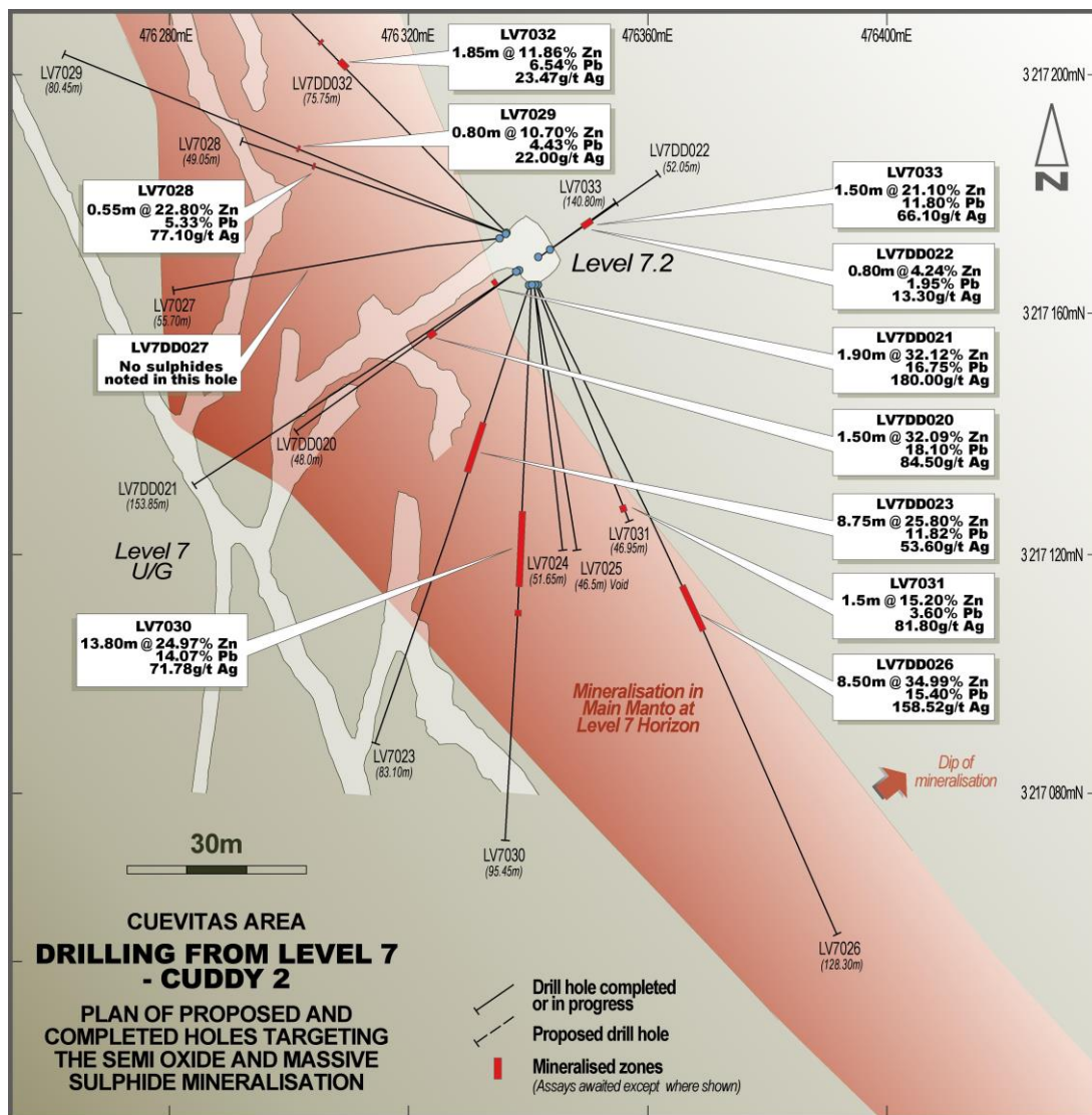
Figure 1. Drilling completed from Cuddy 7.2 with drilling results to date
