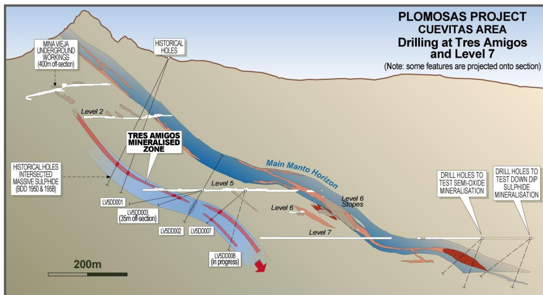
Figure 5. Section view of the Plomosas mine through Cuevitas area (A-A') showing the Tres Amigos zone, historical drilling and the drilling planned for Main Manto Horizon below Level 7.
