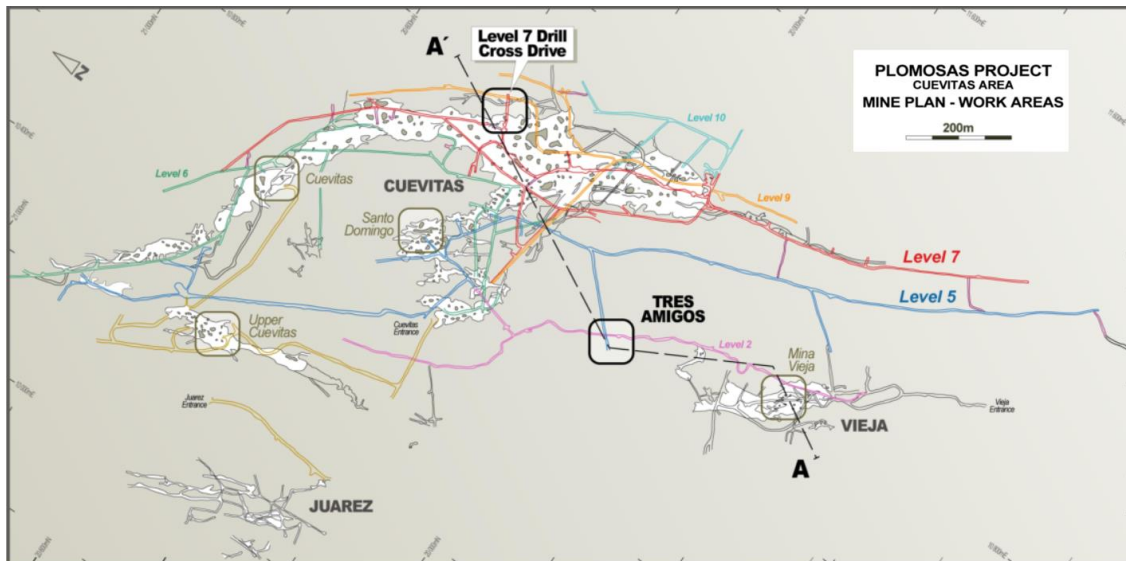
Figure 4. Plan view of the Plomosas mine showing location of the cross section in Figure 6 (trace A-A') and work areas referred to in the text including Level 7 access for drilling the Main Manto Horizon deeps.
