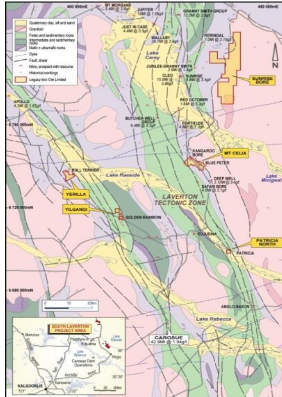
Figure 1: South Laverton Gold Project – Mt Celia
