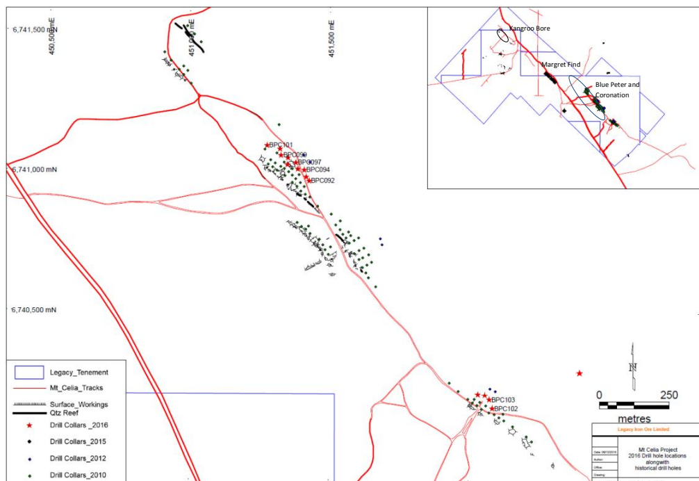
Figure 3: Blue Peter & Coronation Prospect – August 2016 Drill hole location along with historical drilling.
