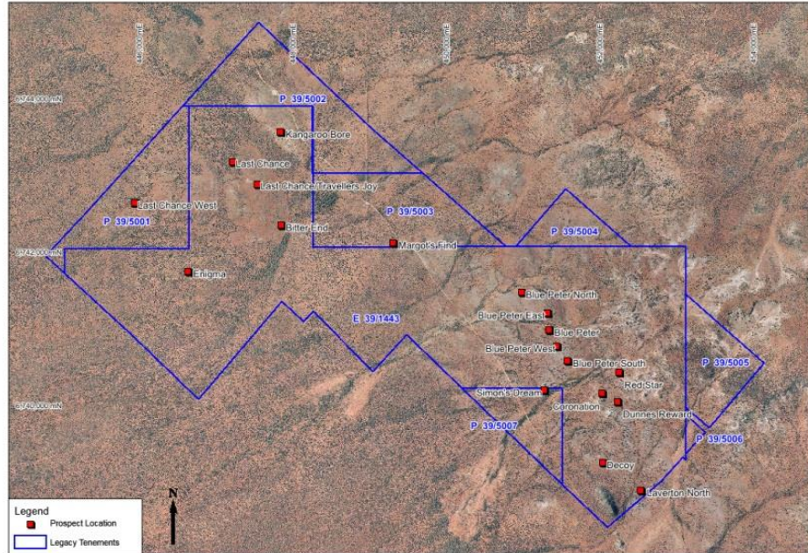
Figure 2: Mt Celia Project- Aerial image showing Blue Peter, Coronation and other prospects
