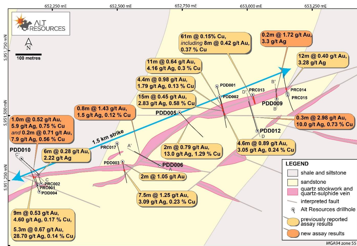
Figure 8. Map of previous and new drilling at the Tom's Vein area of Kidman. New intercepts (from 2016) are shown in orange.
