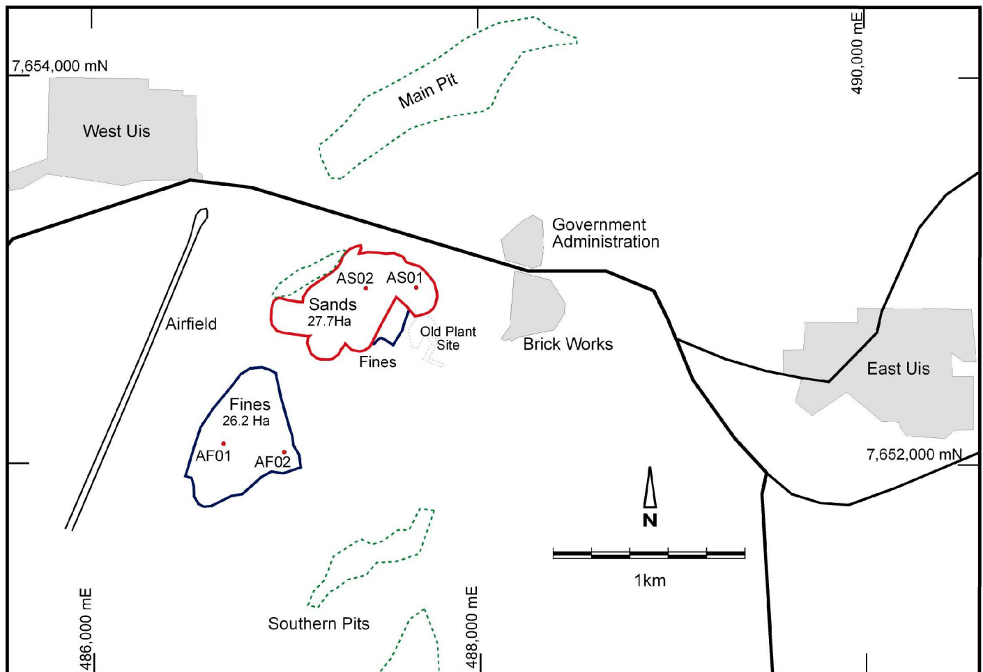
Figure 2 | Project Layout
