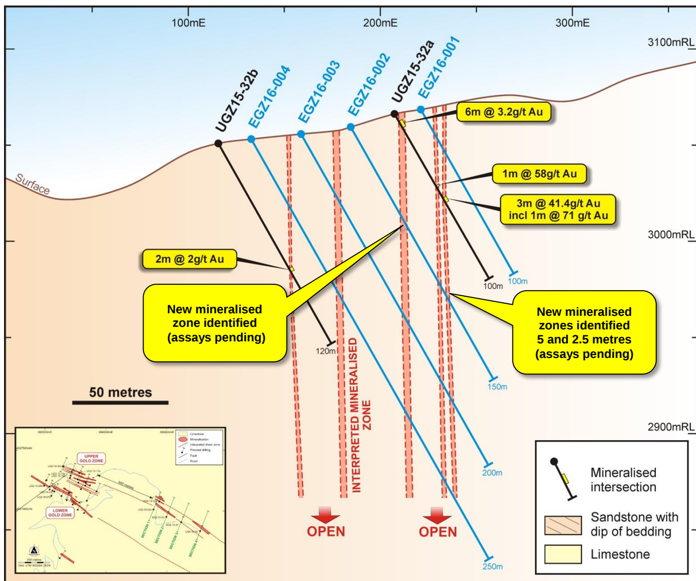
Figure 2: Schematic Cross Section 1 showing planned holes in blue and existing holes in black. Drill hole EGZ16-002 has been completed and EGZ16-003 is underway.
