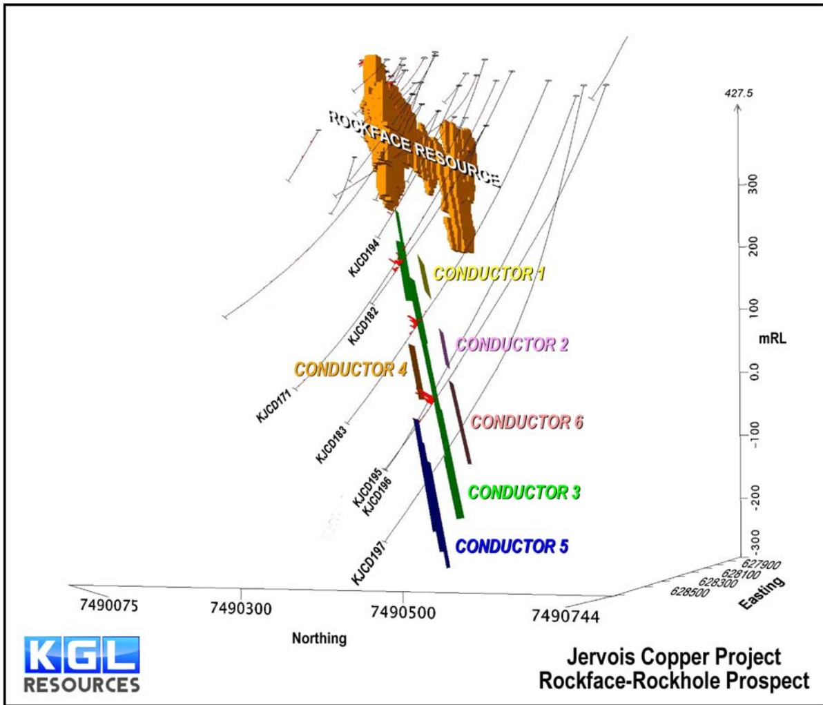
Figure 2 Rockface DHEM plates (view angle 254 deg)
