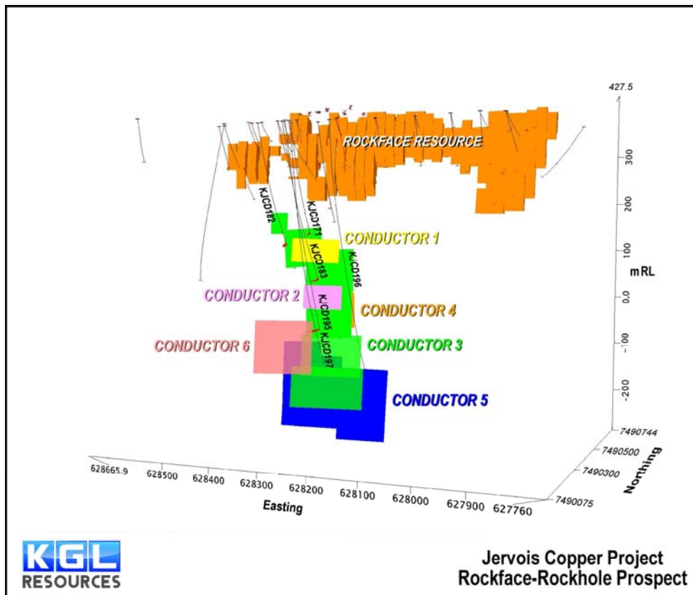
Figure 1 Rockface DHEM Conductors (view angle 158 deg)
