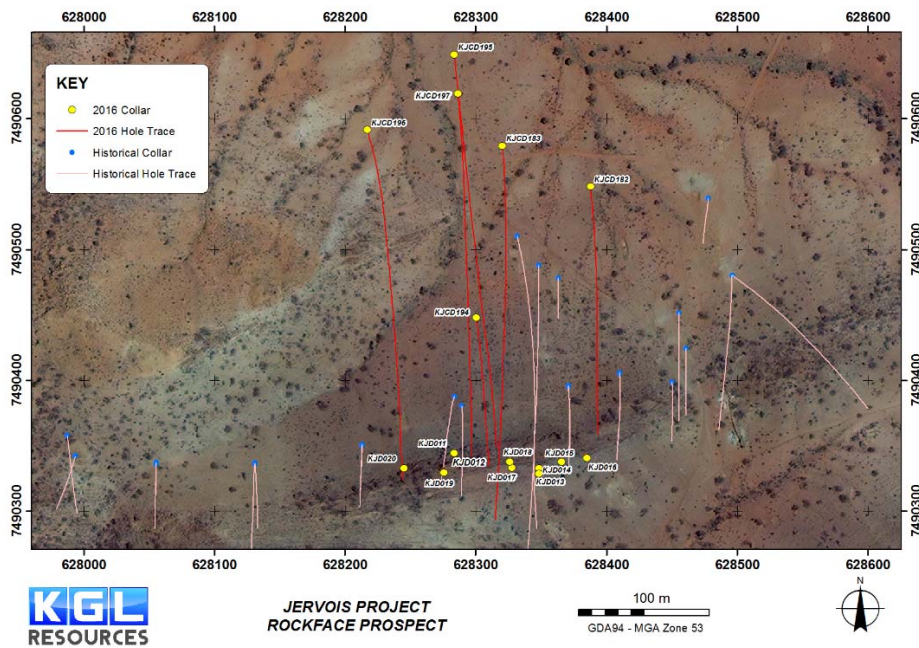
Figure 4 Plan of Rockface drilling
