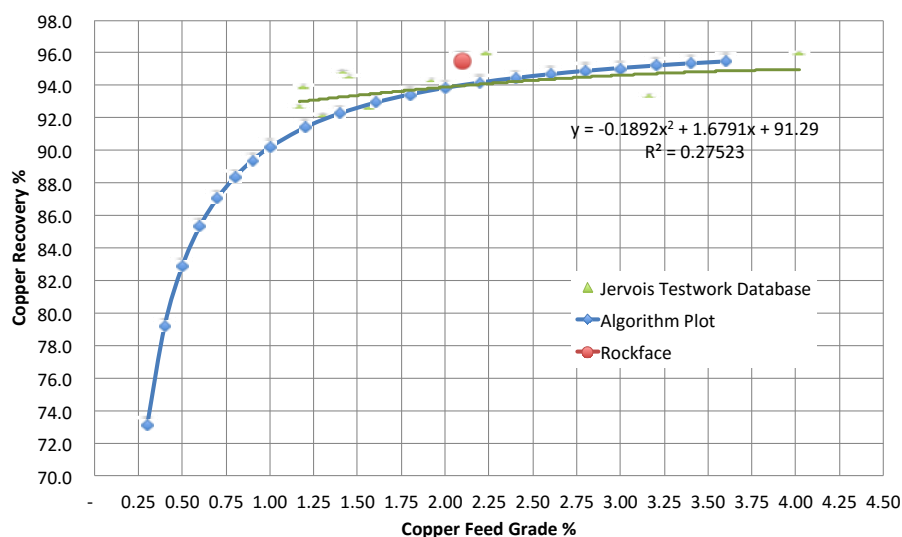
Figure 3 Copper Feed Grade vs. Copper Recovery - Sulphide Ores
