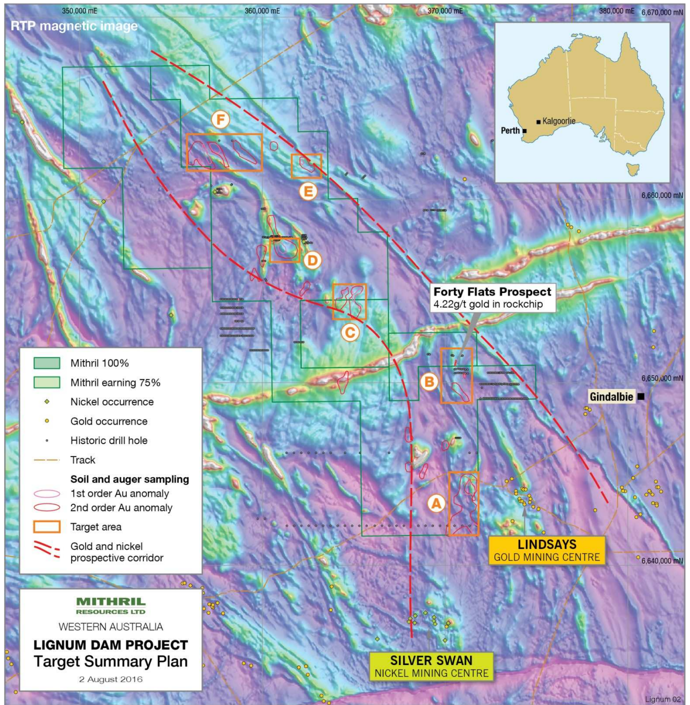
Figure 2: Lignum Dam Project Target Summary Plan showing location of priority targets, geochemical anomalies and historic drill collars on a RTP magnetic image background
