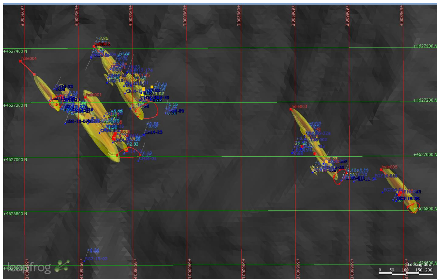
Figure 1: Modelled mineralised lodes following the NW structural trend (mineralisation is open in both directions). High grade mineralised shoots are interpreted to plunge at 25 degrees to the northwest (Figure 2)
