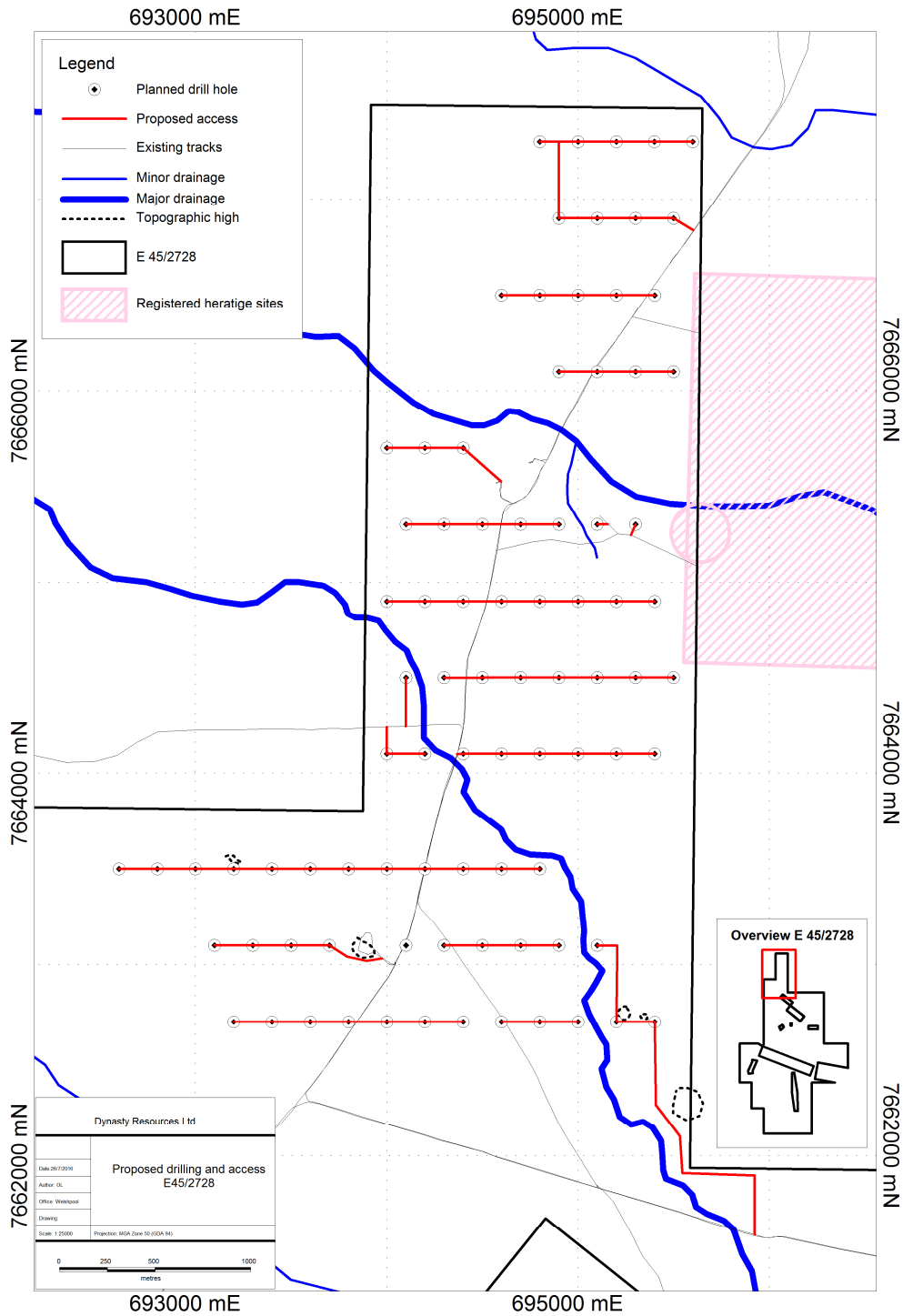
Figure 2 Planned Drilling program
