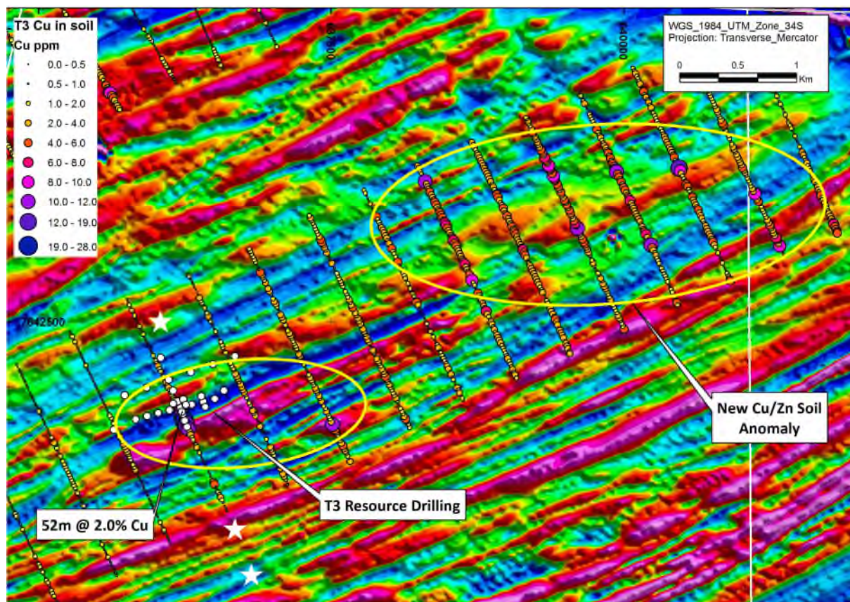
Figure 1: Magnetic image of T3 area showing current resource drilling and large coincident Cu/Zn soil anomaly located ~3.5km along strike. White stars represent 3 deeper drill targets based on interpretation of trial IP data.
