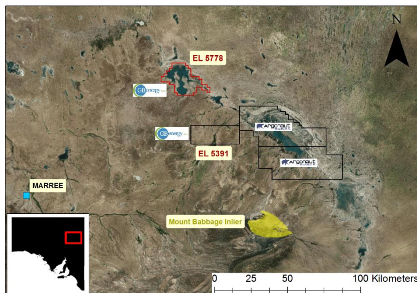
Figure 1: EL 5778 with nearby tenements including GBX-held EL 5391
