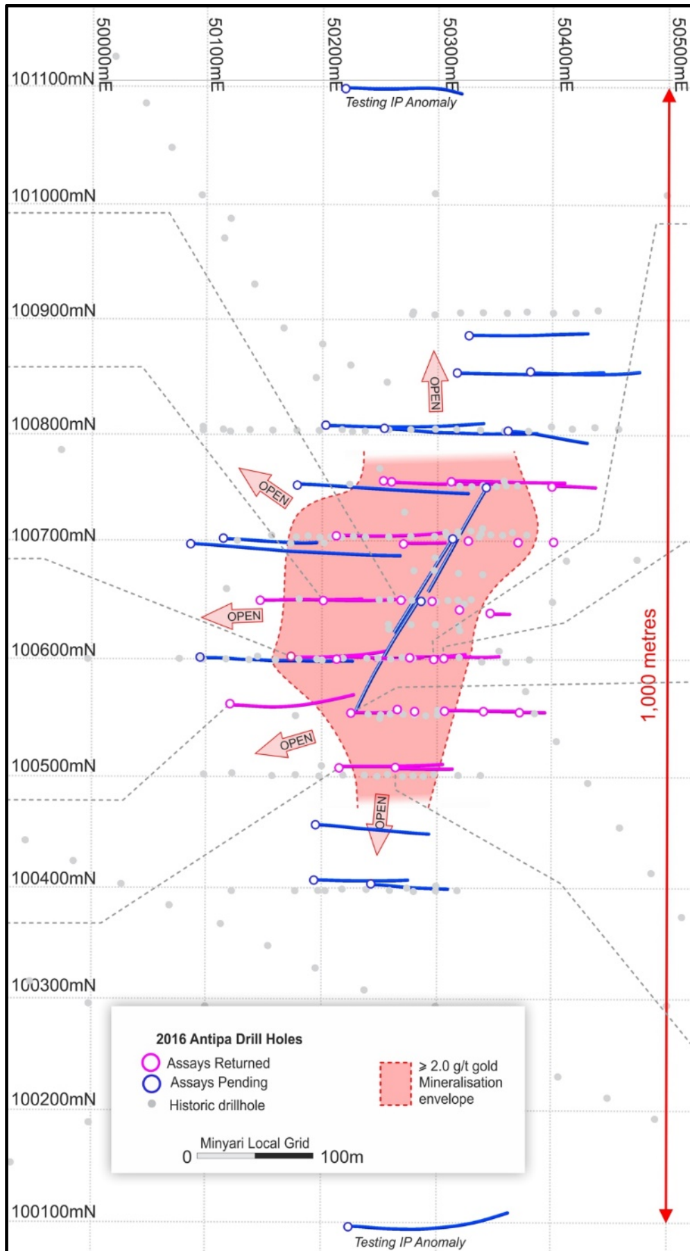
Figure 1: Minyari Deposit plan view showing drillhole locations and plan projection of approximate boundary of \geq 2.0 g/t gold mineralisation. Note: 2016 Phase 1 RC drillholes purple = Assays Returned, blue = Assays Pending.
