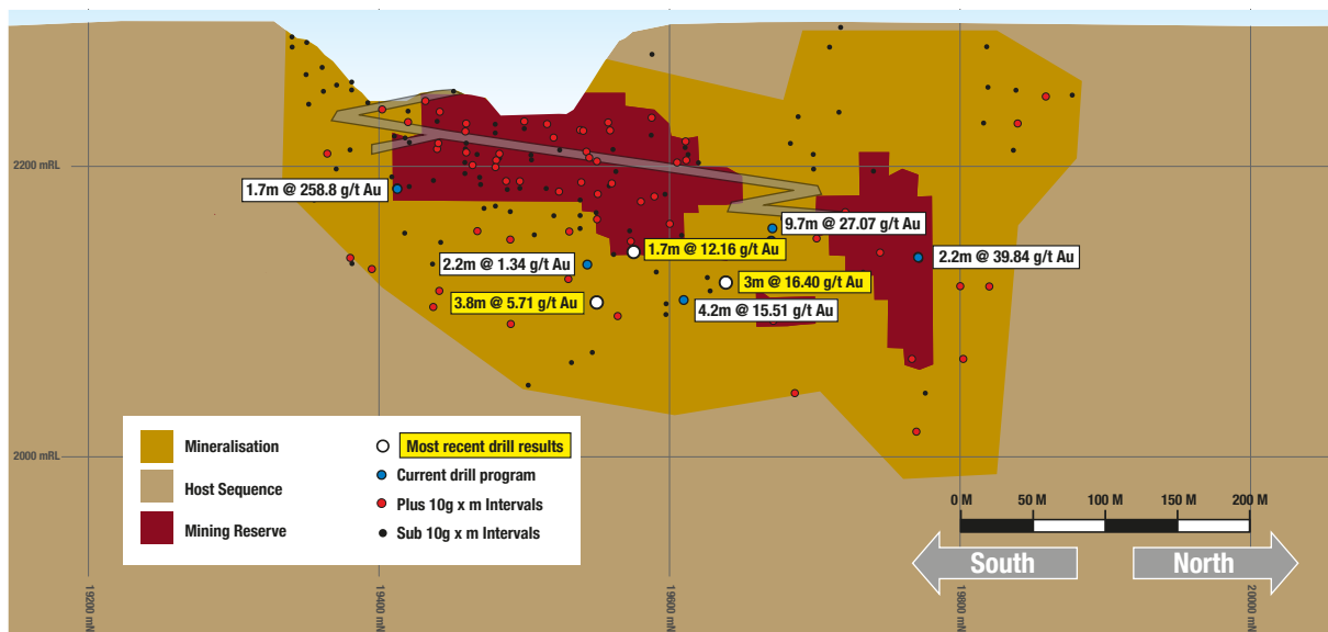
Hall and Anderson Lode Schematic Long Section
