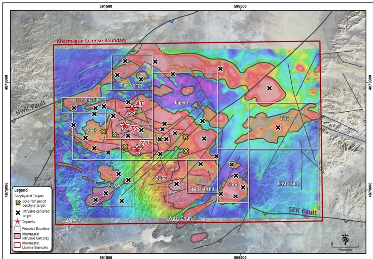
FIGURE 2: Kharmagtai porphyry copper-gold district showing Altan Tolgoi, Tsagaan Sudal and Zesen Uul deposits. Ground magmatic map showing the newly generated drill targets defined following reprocessing of the extensive geophysical database.
