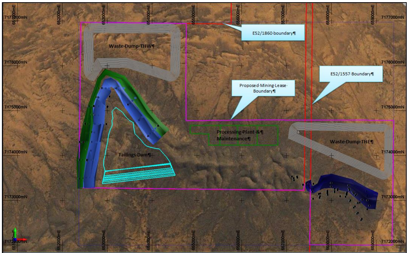
Figure 3. Mining lease location (magnetite deposits shown in blue and green).
