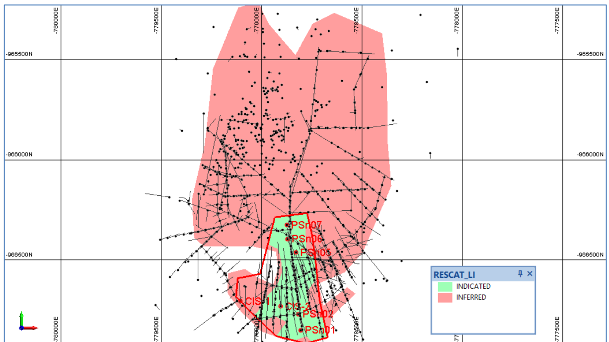
Figure 1: Plan view of Cinovec Project drillhole locations, historic underground workings, Li Indicated and Inferred Resource. Outlined in red is the area within which data were reviewed for the resource upgrade.
