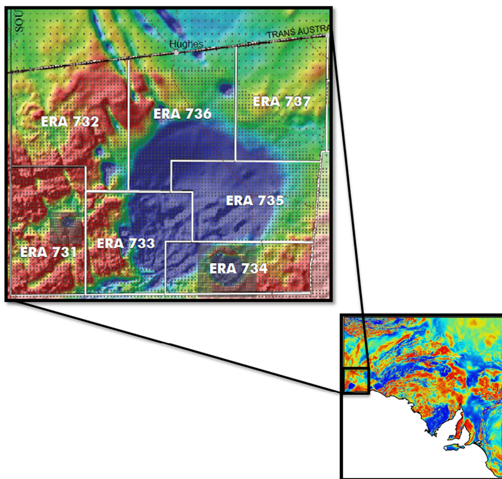
Figure 1: Coompana Project Location on background regional aeromagnetic image.
