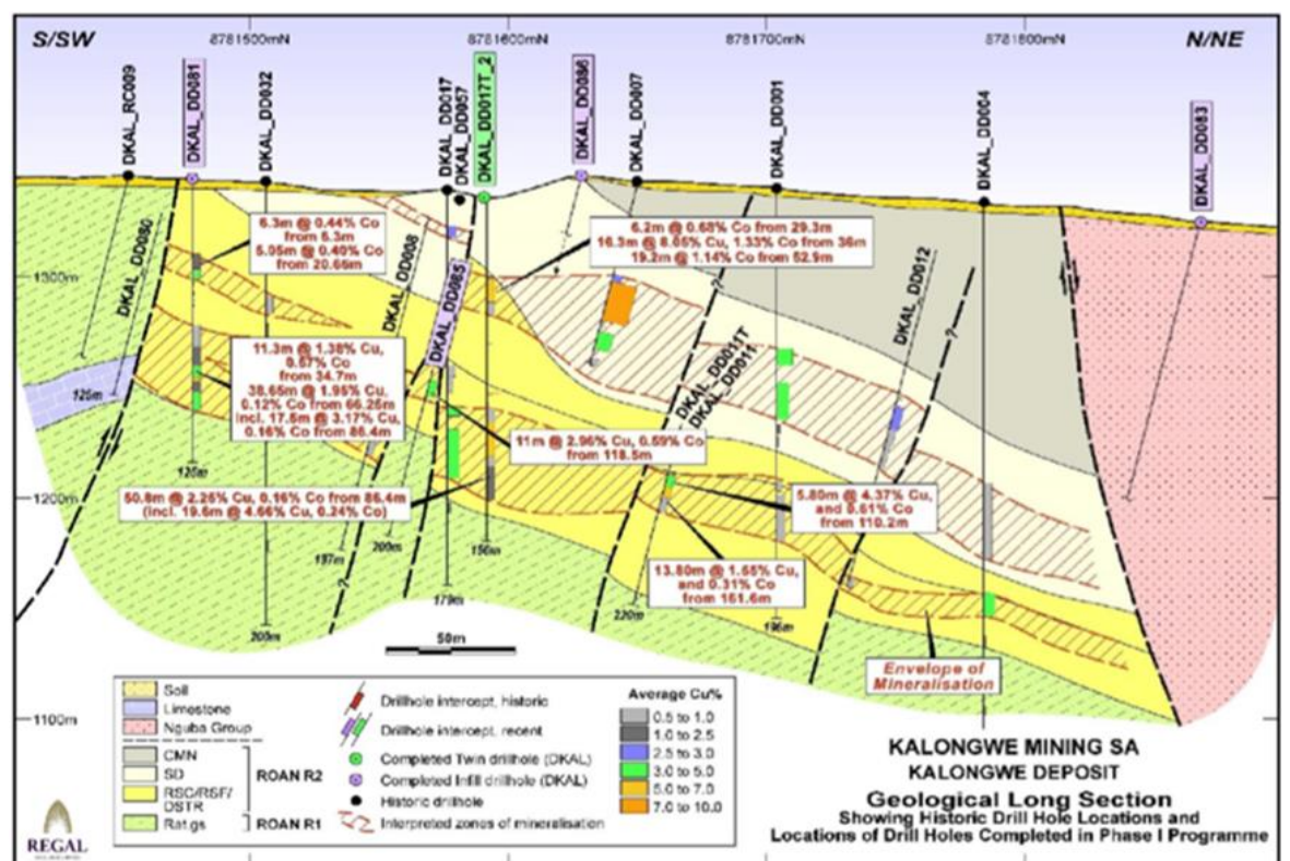
Figure 12 Geological Long Section of the Kalongwe Cu-Co mineralisation
