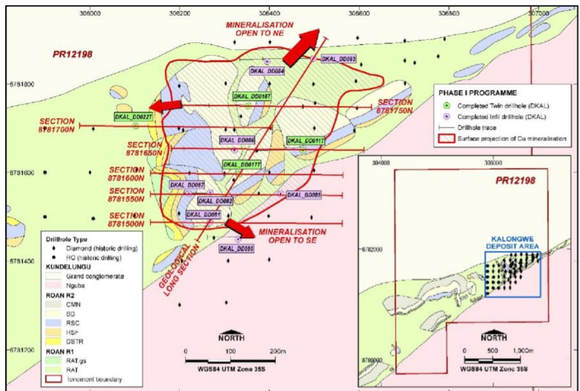
Figure 11 Geological Map of the Kalongwe Cu-Co Project Area and Location of Drill Holes Completed in the Phase I Program
