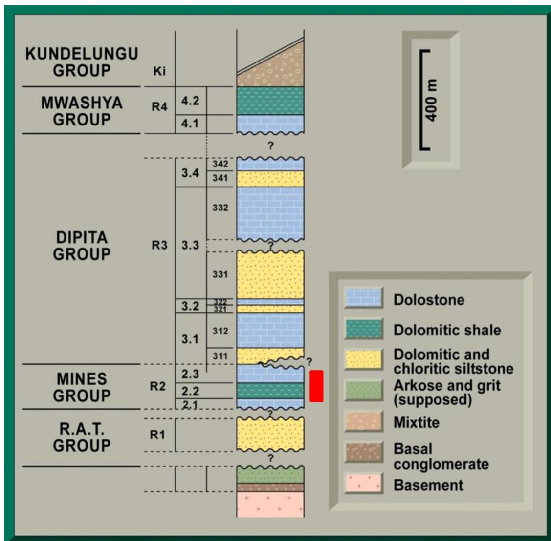
Figure 7 Lower Part of the Katanga Stratigraphy.
