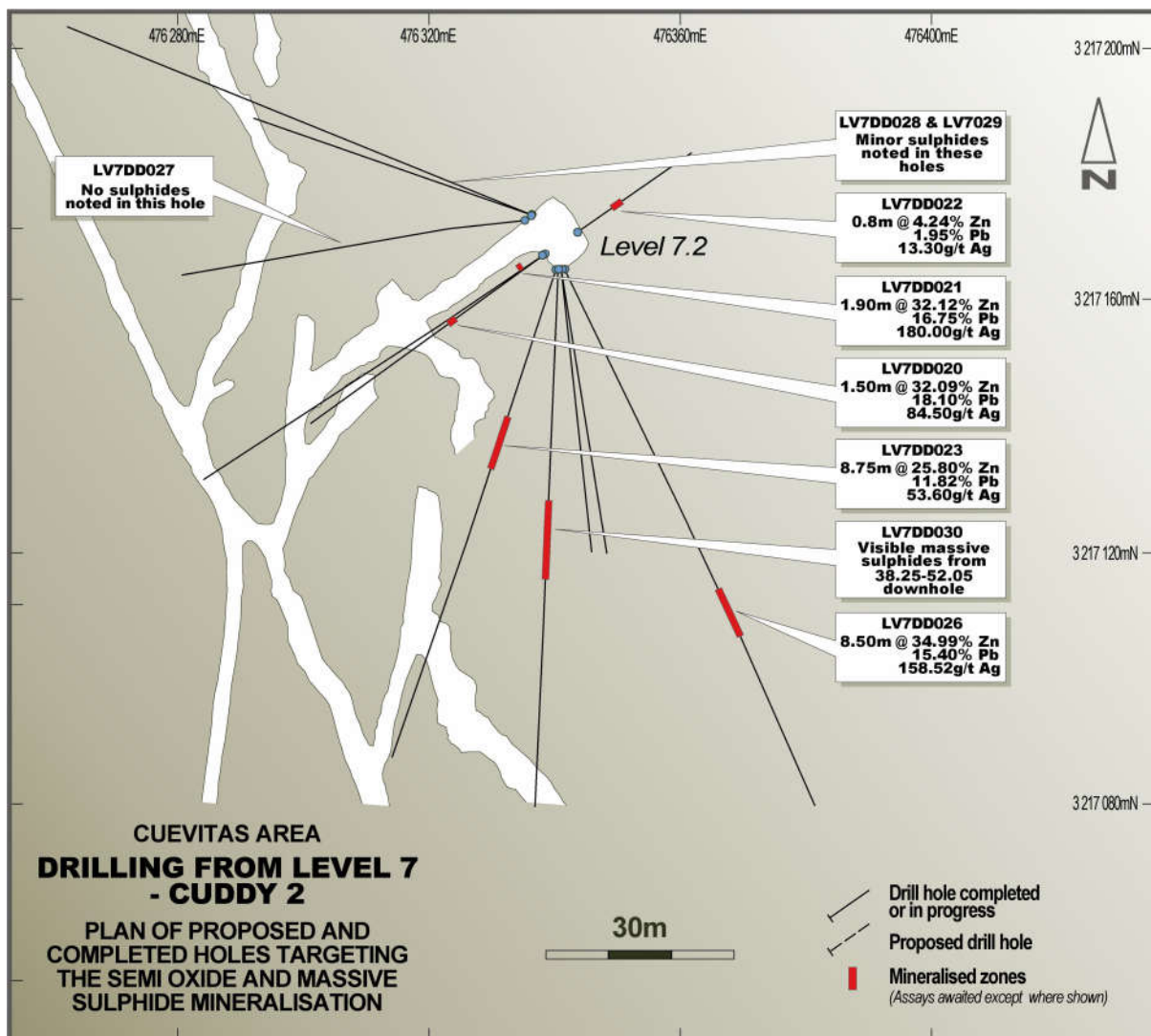
Figure 2. Drilling completed from Cuddy 7.2 with drilling results to date
