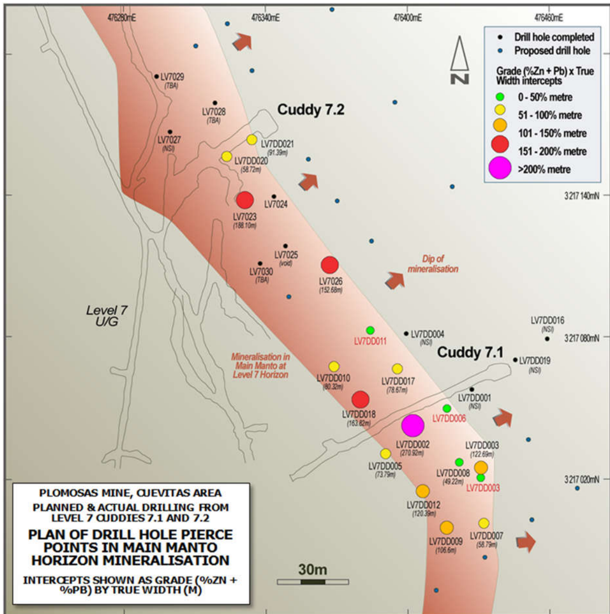
Figure 5. Planned and actual pierce point of holes drilled from Cuddies 7.1 and 7.2 showing strength of intercepts obtained.
