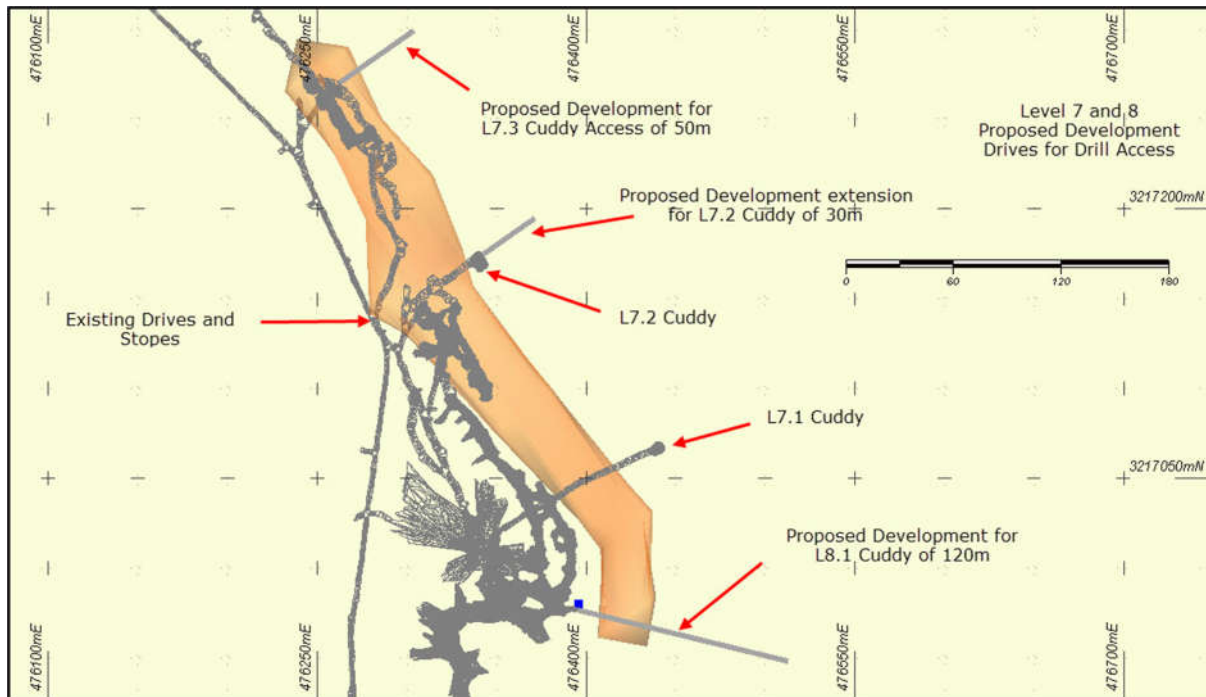
Figure 1. Proposed development locations from Level 7 opening up the down dip and northern and southern extensions of the mineralisation.
