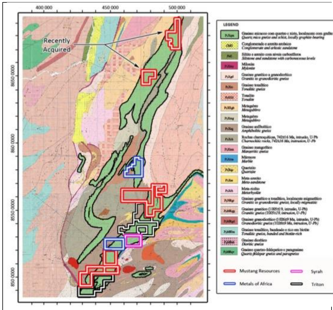
Figure 2. Mustang's Balama Graphite Project, regional geological map depicting the graphitic schist strike through the exploration concessions
