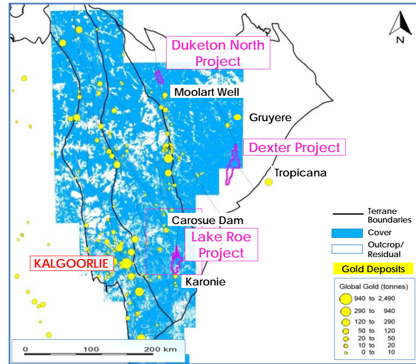
Gold Deposits in WA's World Class Eastern Goldfields
