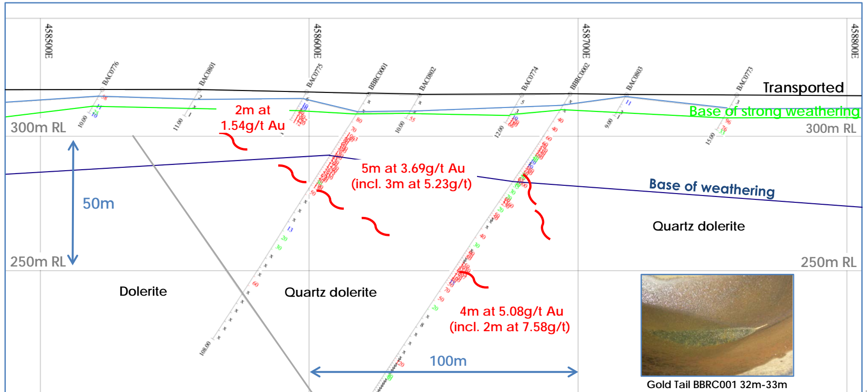
Bombora RC Northernmost Drill Cross Section (looking north; downhole grades in ppb)
