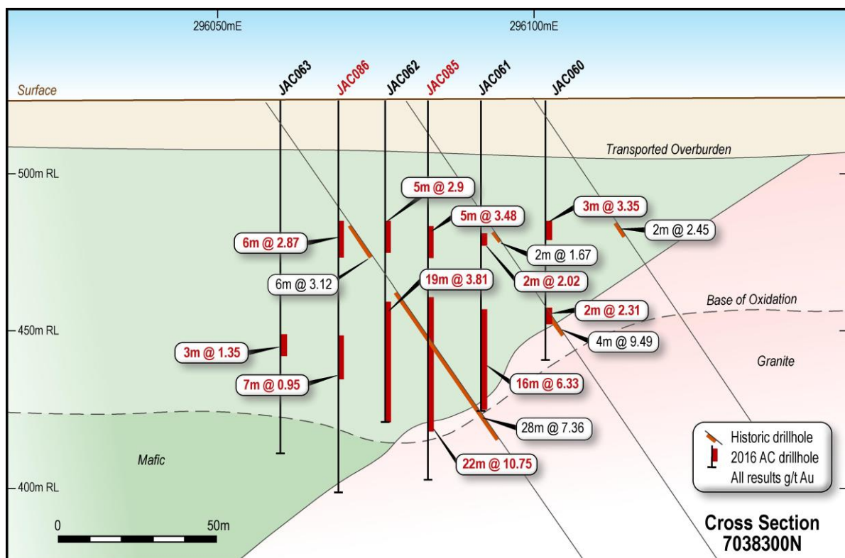
Figure 4: Julius Cross Section 7038300N
