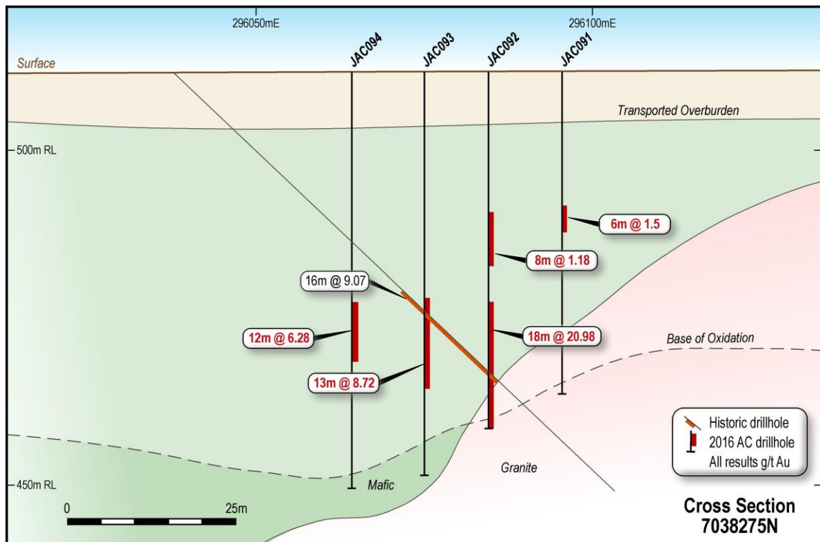
Figure 3: Julius Cross Section 7038275N
