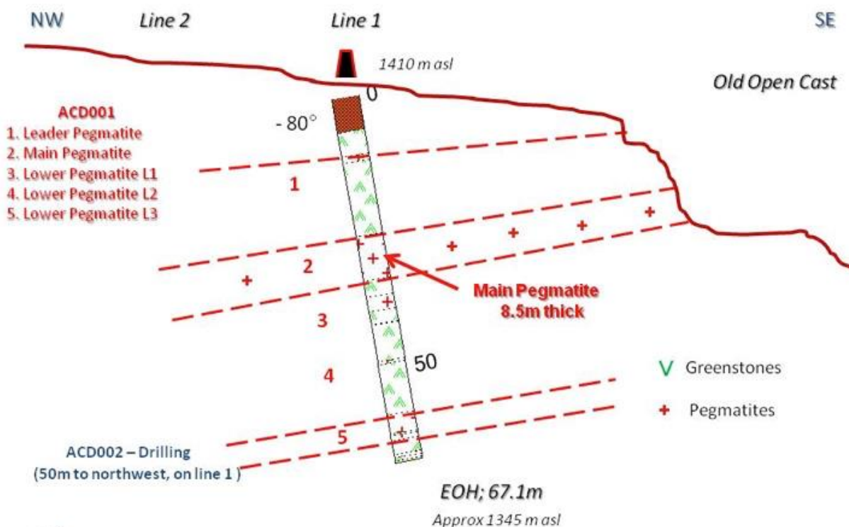
ACD001 – Schematic Drill Section – looking NE
