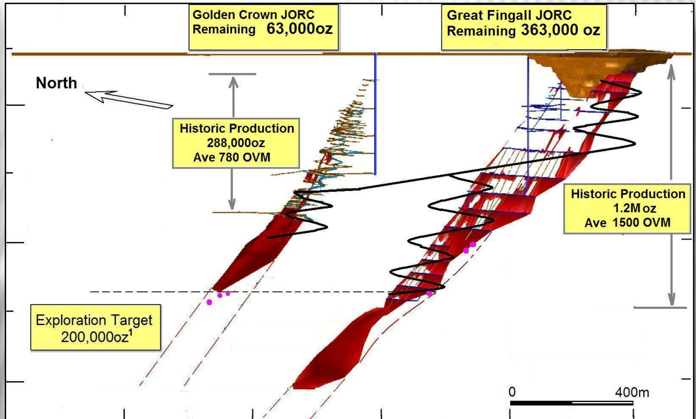
Conceptual decline access
