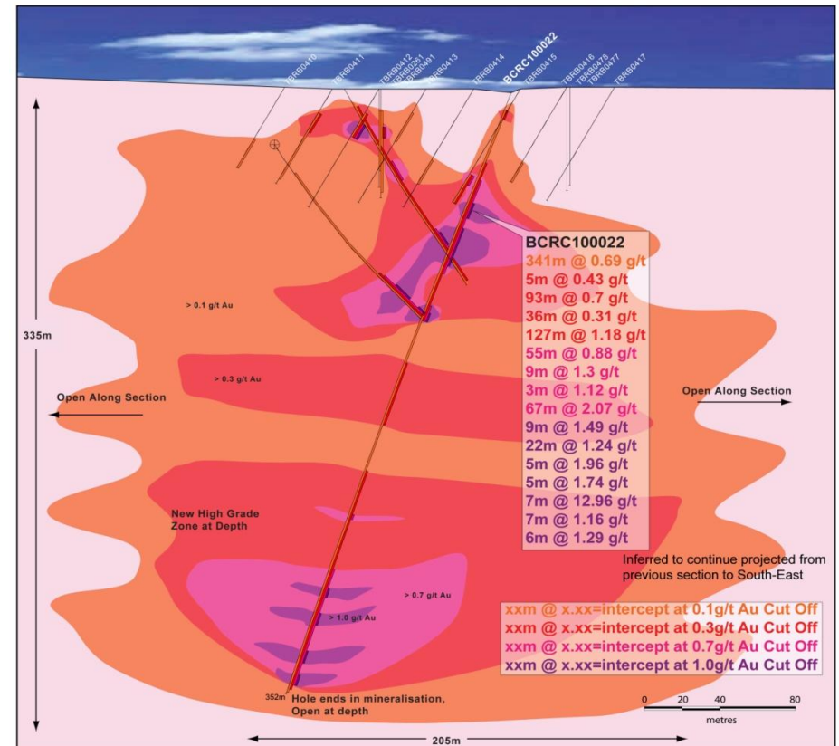
Cross-Section G
