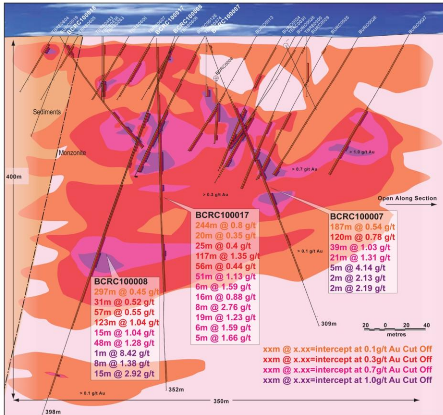
Cross-Section D
