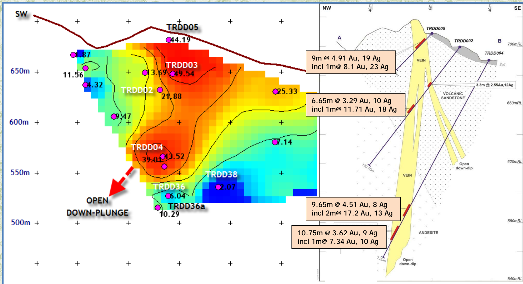
WEST SENTUL VEIN LONG SECTION GOLD GRADE (g/t) x VEIN INTERCEPT (m)
