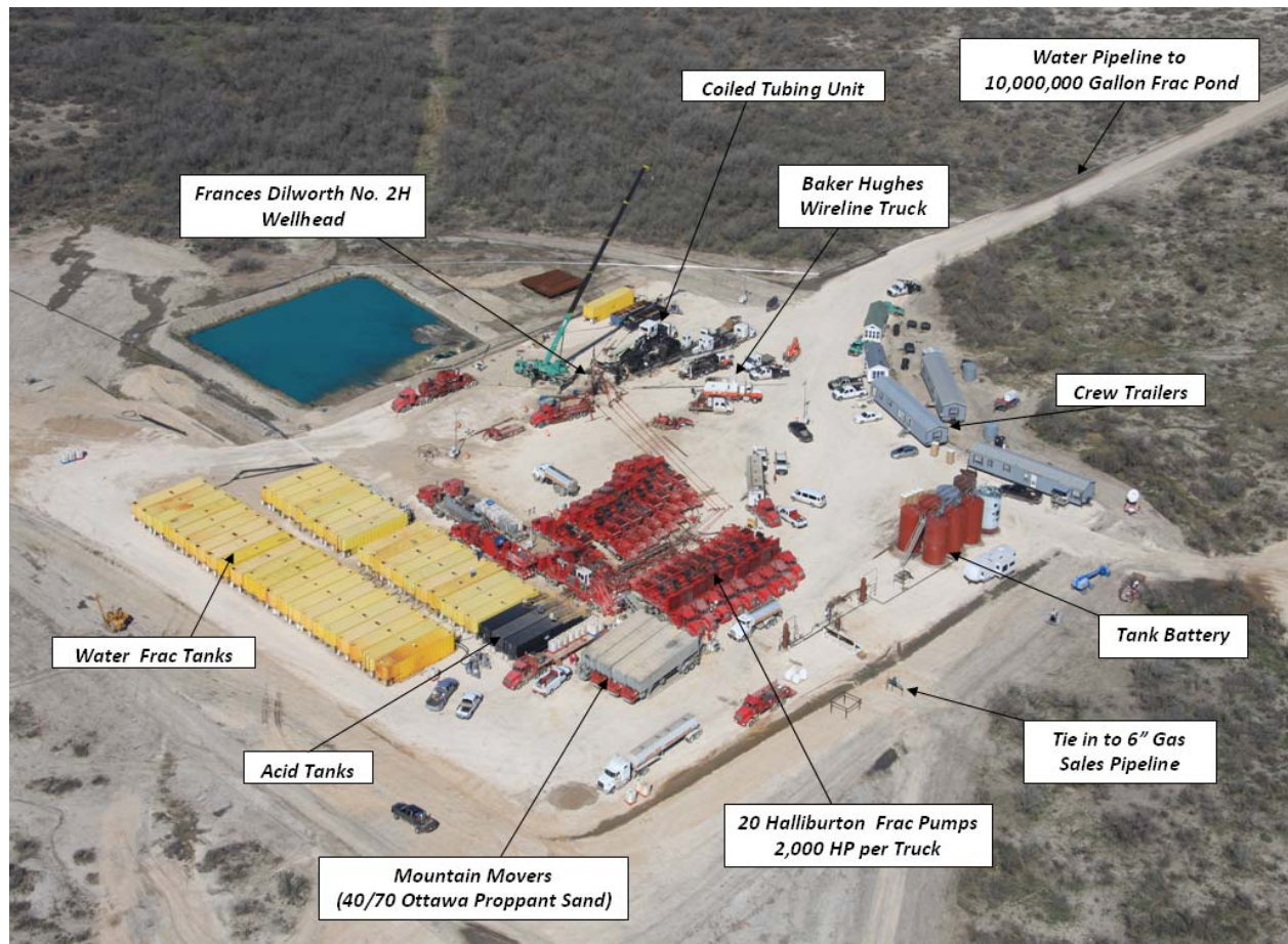
Aerial photograph of fracture stimulation operations at the Frances Dilworth No. 2H.
