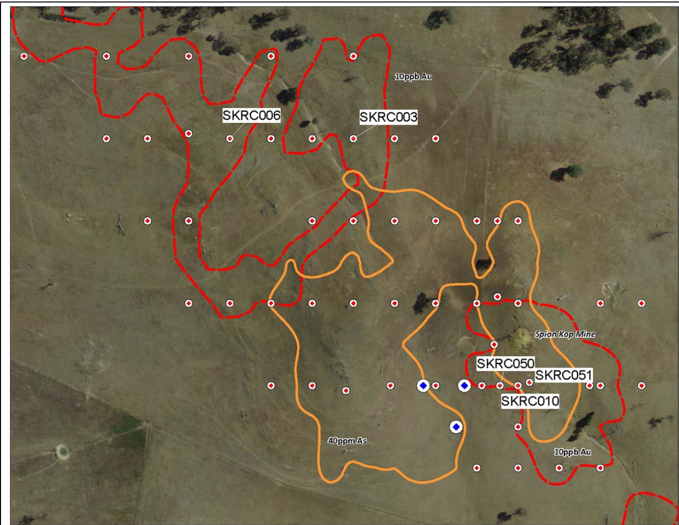
Figure 2 :Spion Kop Prospect – proposed diamond core holes (blue circles), RC drillholes with significant gold mineralisation (labelled), gold and arsenic geochemical anomalies and RC drillhole locations (red circles)
