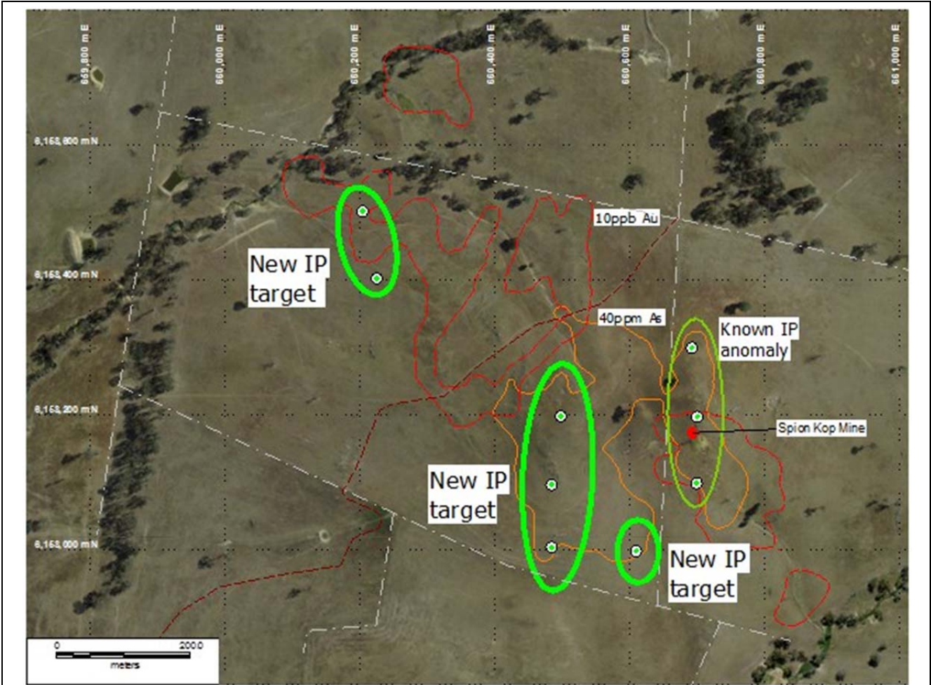
Figure 1 : Boorowa Project. Spion Kop Prospect - gold and arsenic geochemical anomalies and IP targets
