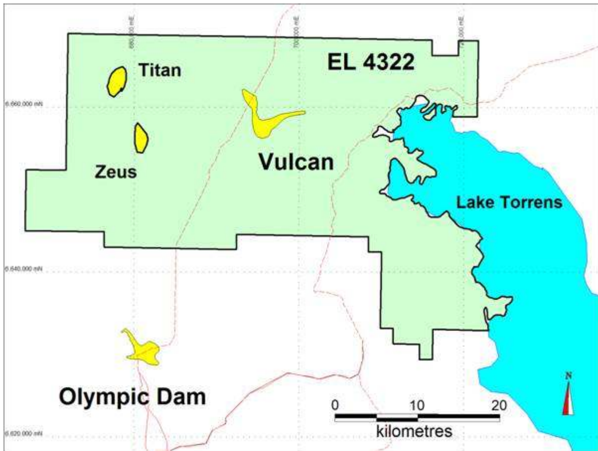
Figure showing Tasman Resources Ltd Exploration Licence 4322, and the location of the Vulcan Project target area (together with Zeus and Titan Prospects) and the Olympic Dam Ore Deposit.
