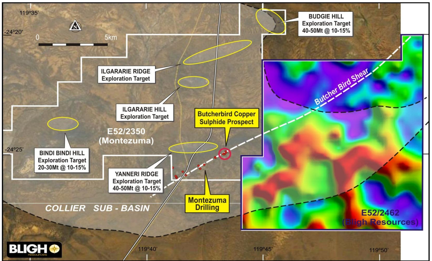
Kumarina Project - 30metre Conductivity Depth Slice Image
