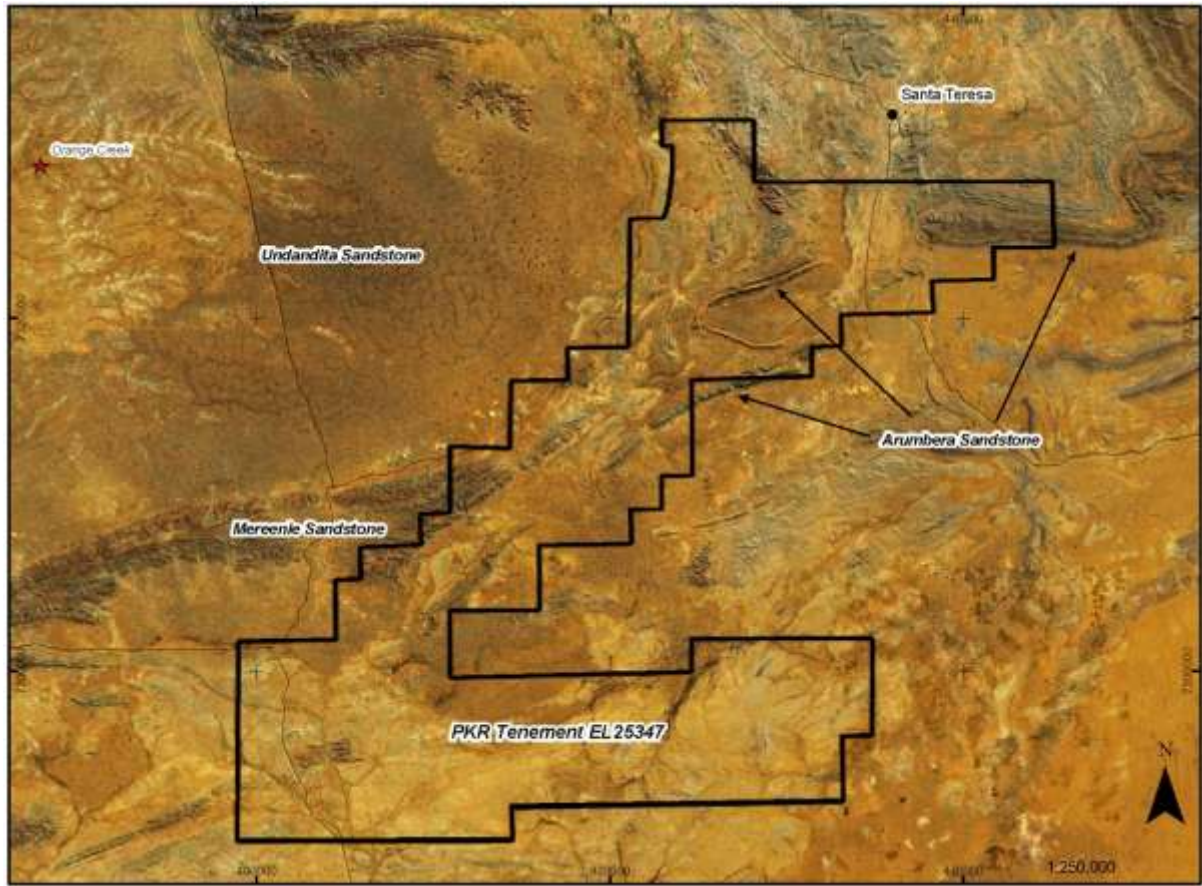
Figure 2. Google earth image of the tenement depicting the ridges formed by the resistant weathering Arumbera and Mereenie sandstone units.
