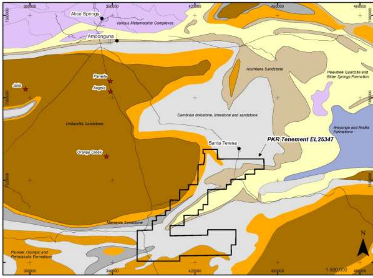
Figure 1. Location and regional geology map of the Allambi Project – Tenement EL25347. The Allambi Project covers sedimentary rocks prospective for sandstone/roll-front or calcrete uranium mineralisation. Several uranium prospects are hosted within the Undandita Sandstone to the northwest of EL25347.
