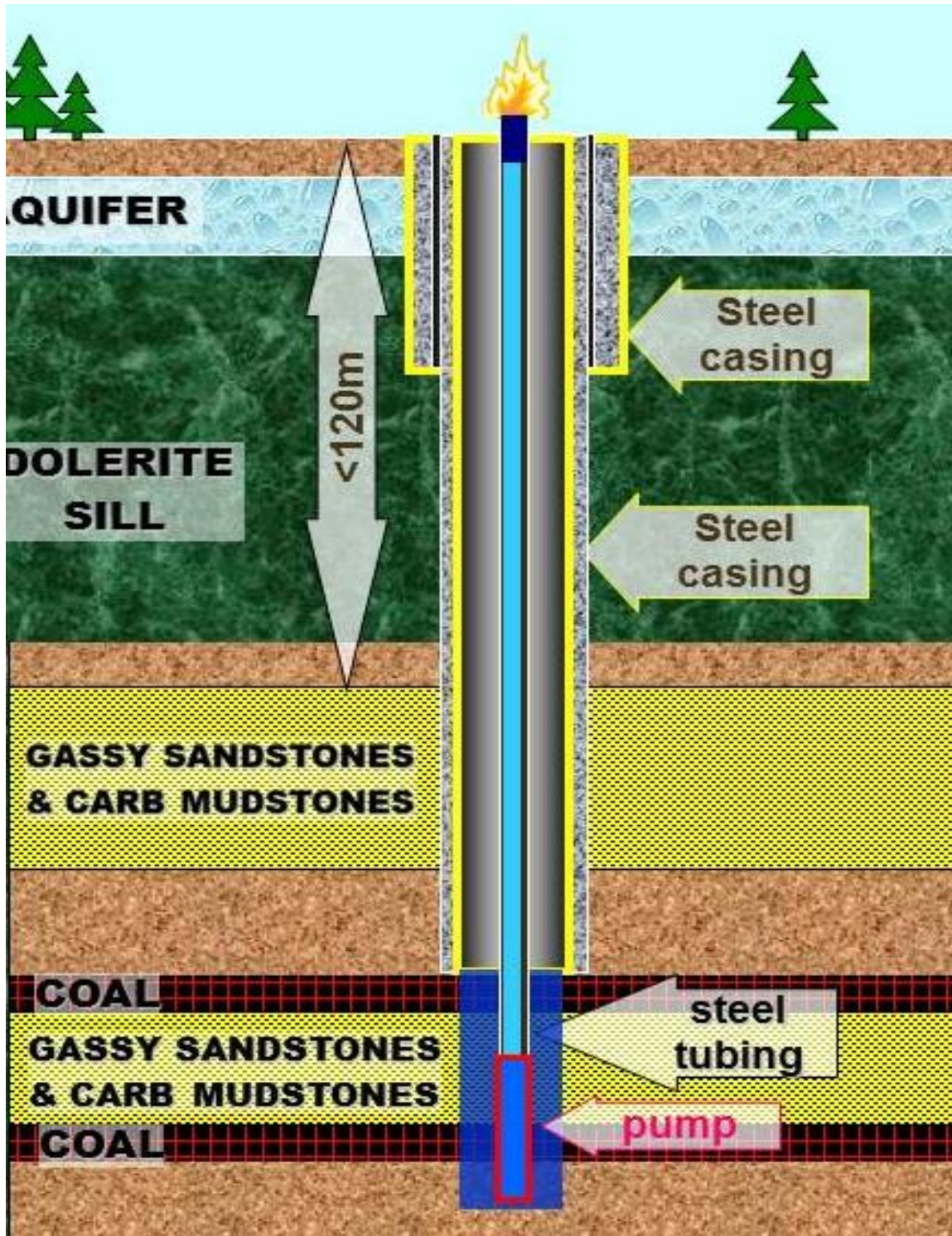
Figure 2: Illustration of gas pilot production well
