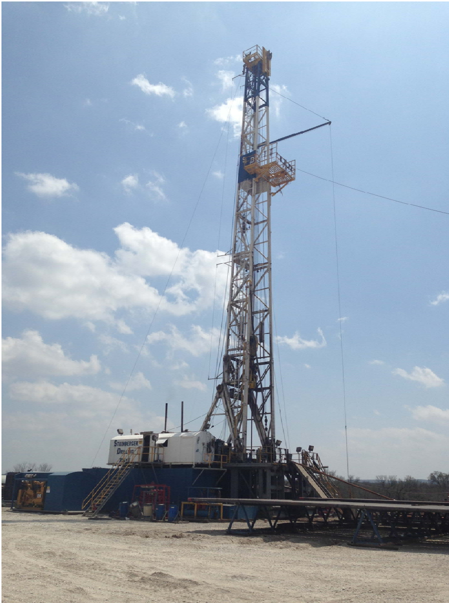
Figure One: Steinberg Drilling Rig # 3 drilling ahead at the third well at Comanche.
