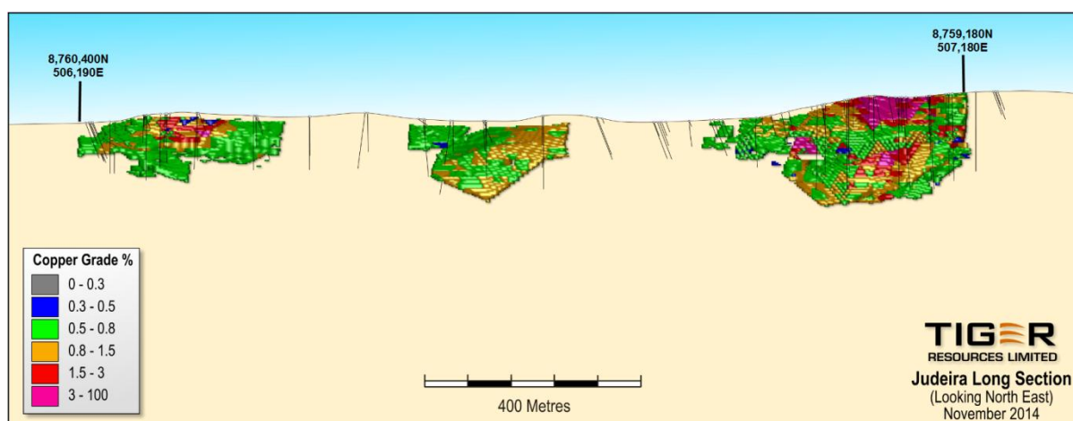
Figure 1: Long section of the Judeira deposit
