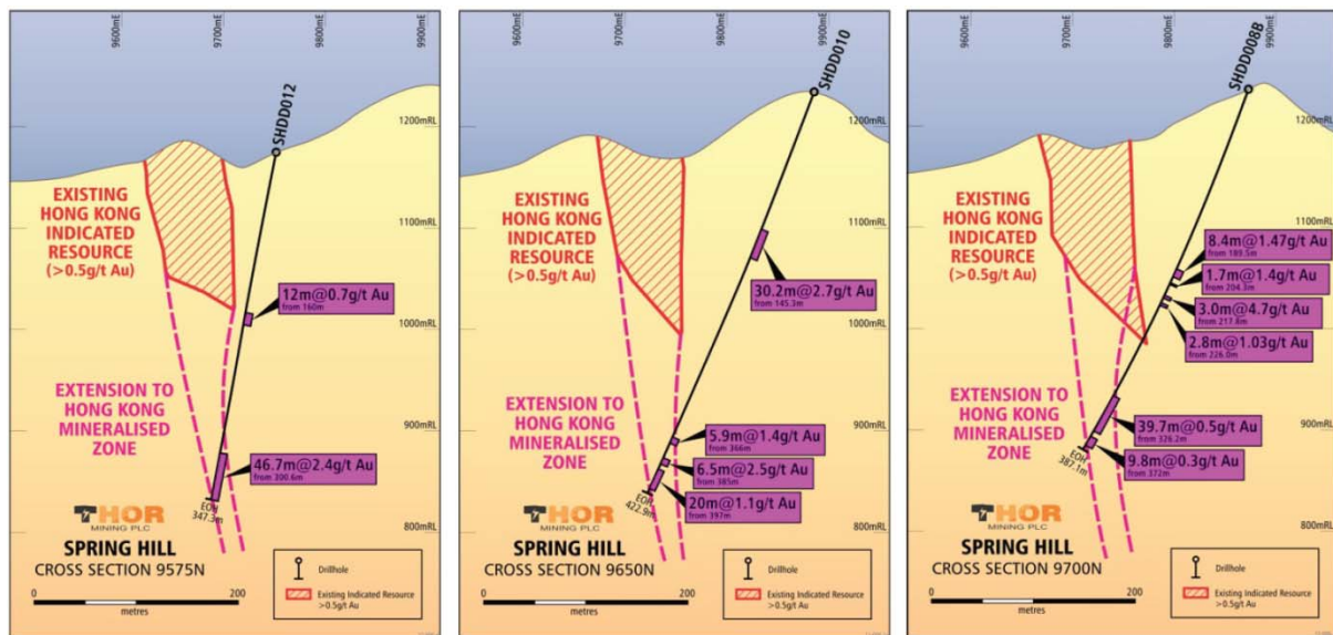
Section looking N at 9575mN
