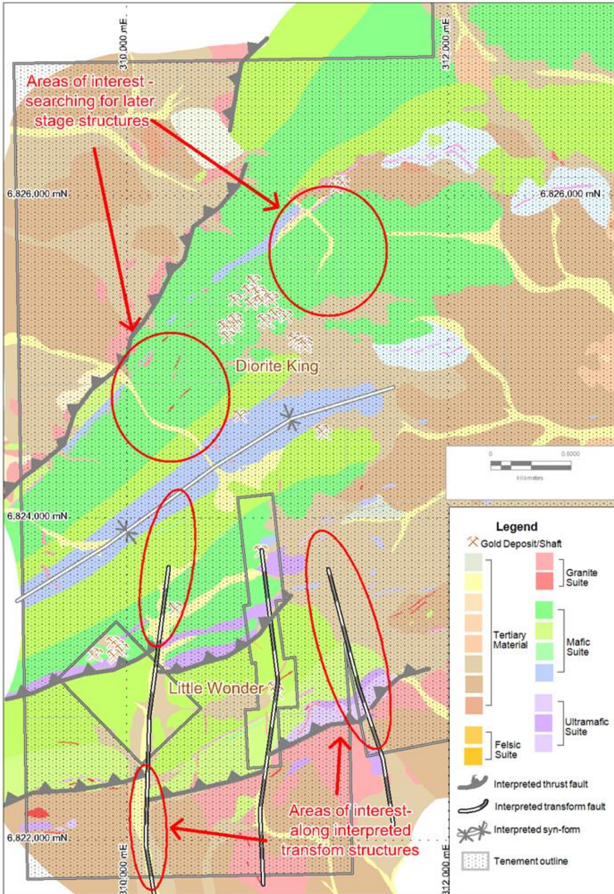
Figure 2: Geological map with structural interpretation and geological areas of interest defined after the mapping program. Coordinates are referenced to Map Grid of Australia (MGA) zone 51.
