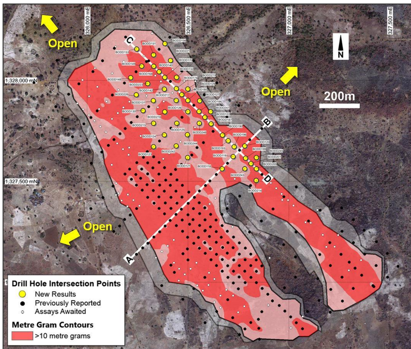
Figure 2 - Natougou drill status plan - showing location of new drill holes and cross sections.
