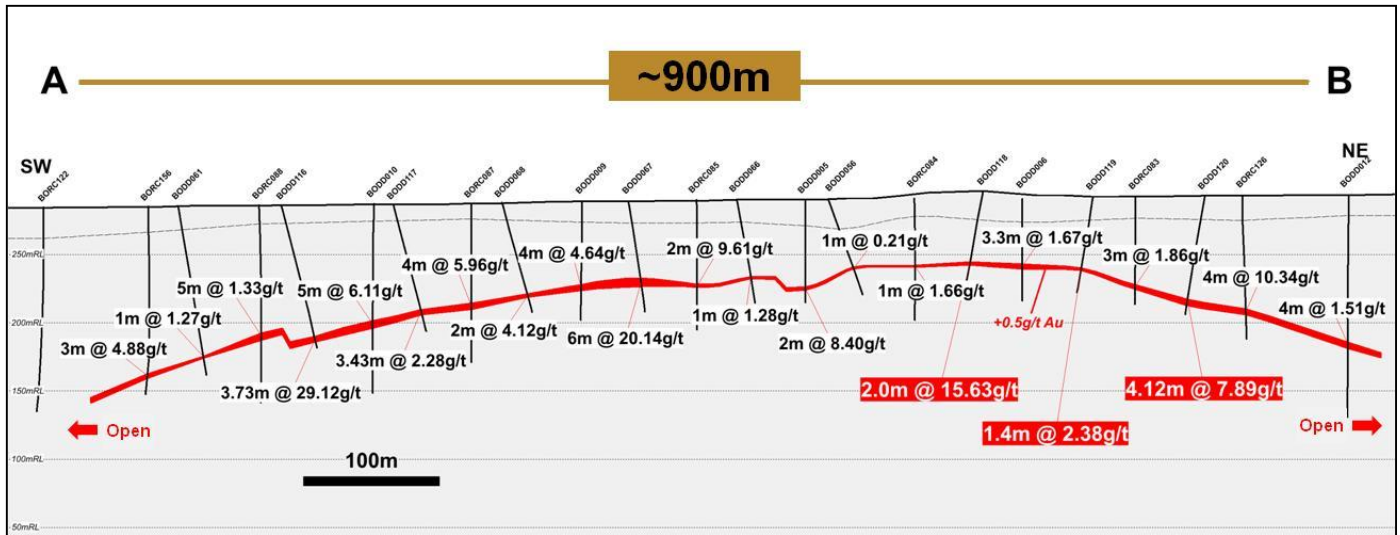
Figure 3 - Natougu cross section "A-B" (new intersections shown in red boxes).
