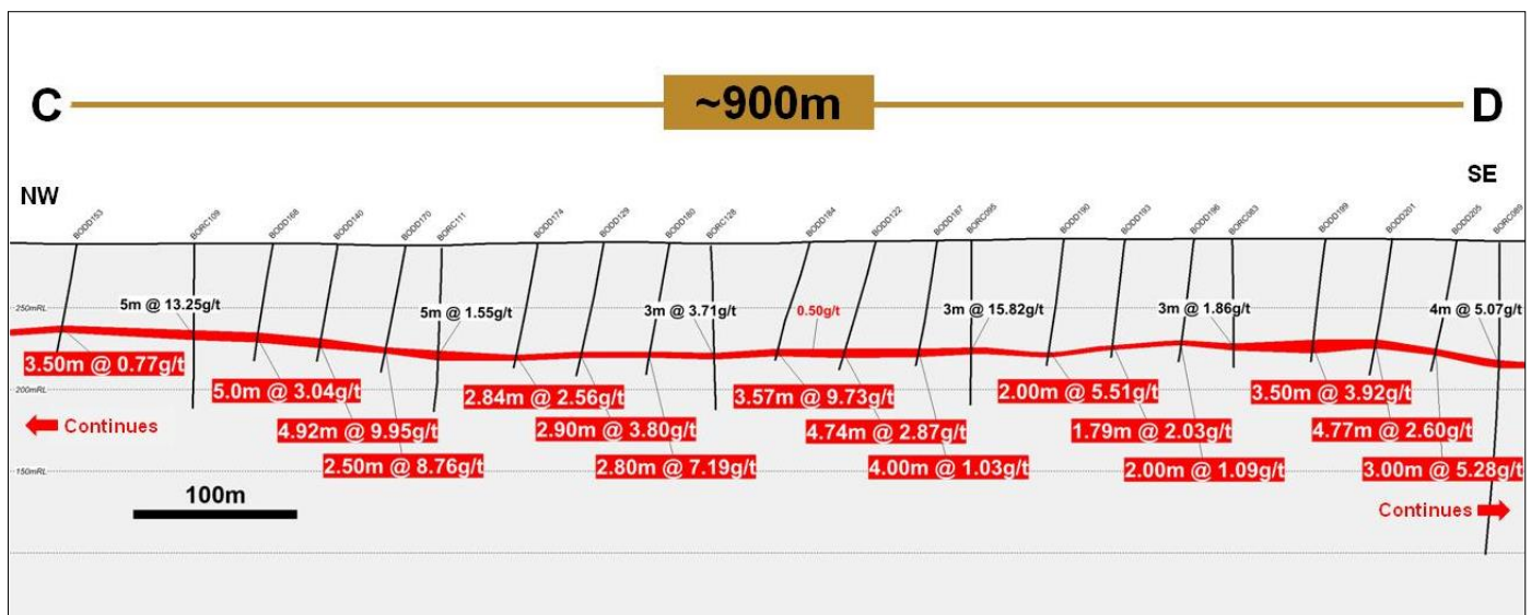
Figure 4 - Natougu cross section "C-D" (new intersections shown in red boxes).
