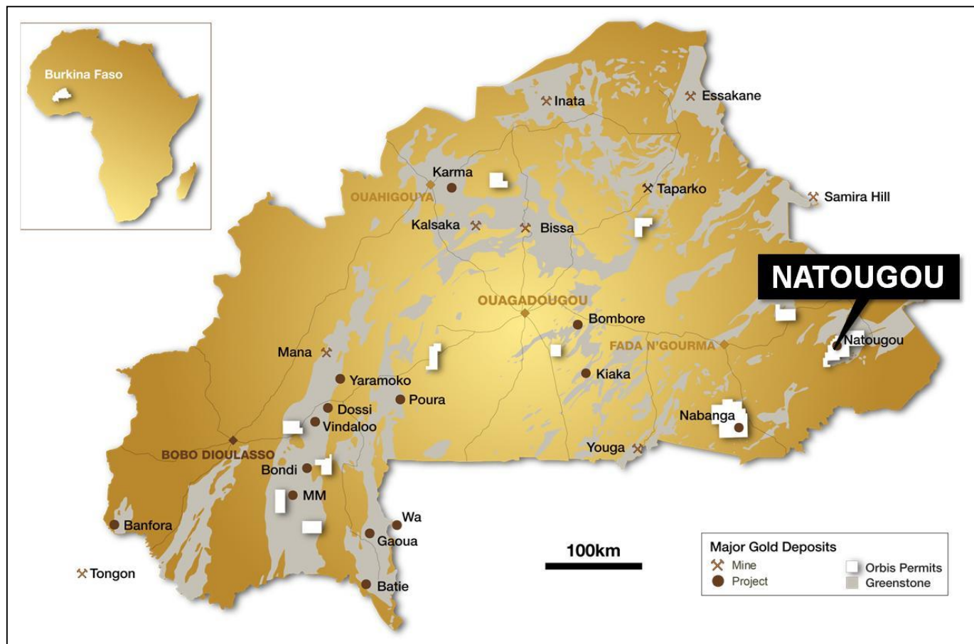
Figure 1 – Natougo location diagram.
