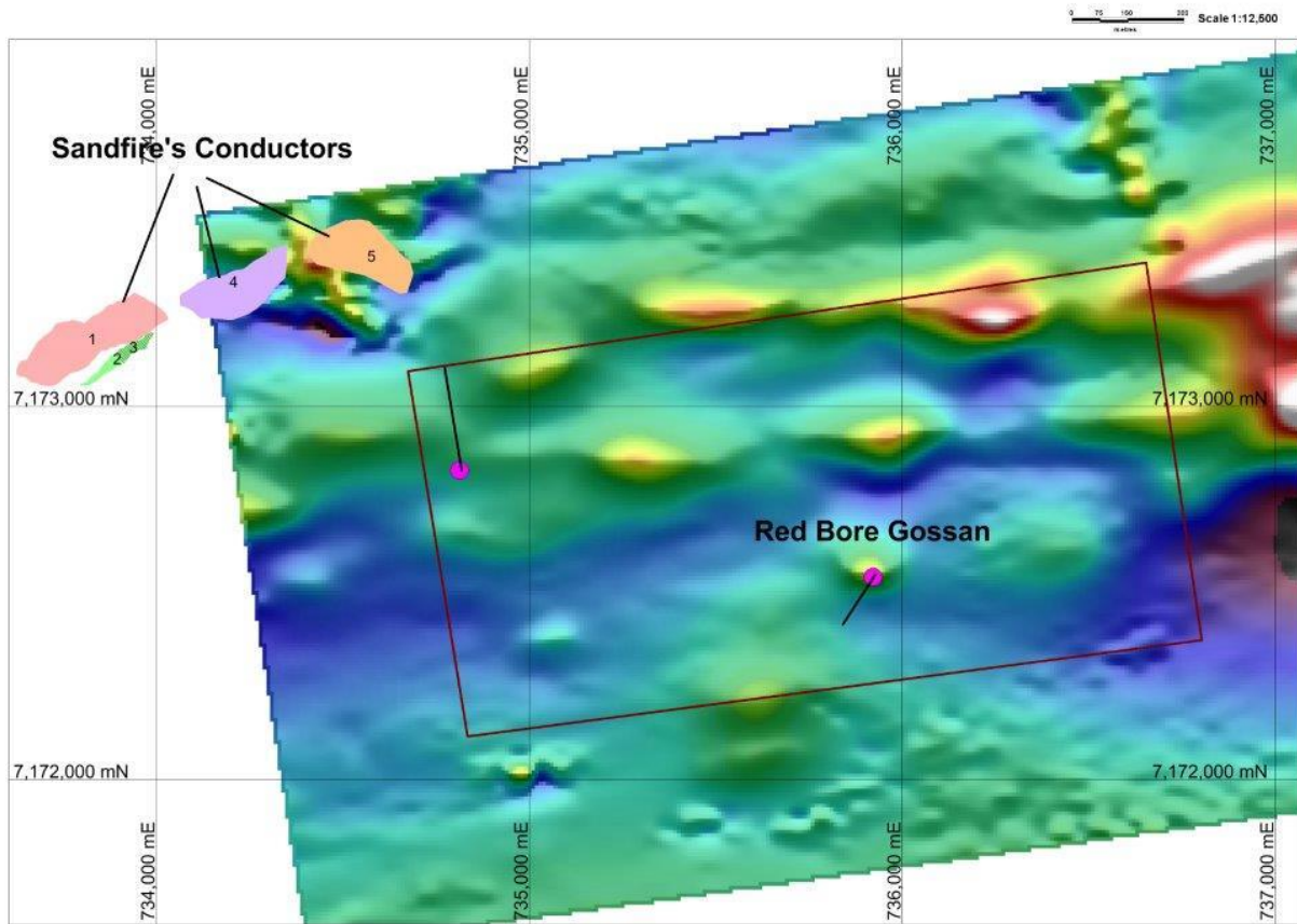
Figure 2: Drill collar location and intended drill azimuth shown on TMI image. Grid spacing is 1,000m. Notional surface traces of the DeGrussa deposits overlain to provide geographical context.
